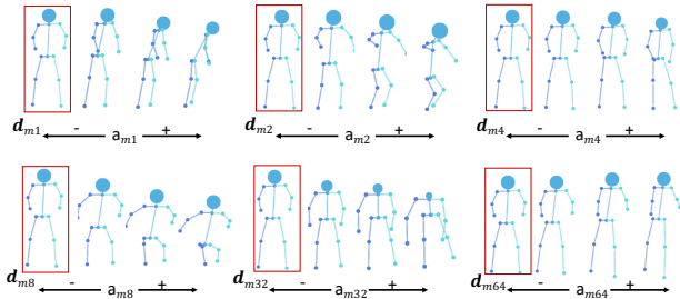
Figure 4. Linear manipulation of six ‘Motion’ directions in \mathbf{D}_v on a skeleton sequence. Results indicate that each direction represents a meaningful motion transformation from a ‘reference pose’ marked in red (e.g., \mathbf{d}_{m8} for squat, \mathbf{d}_{m32} for bending over).
