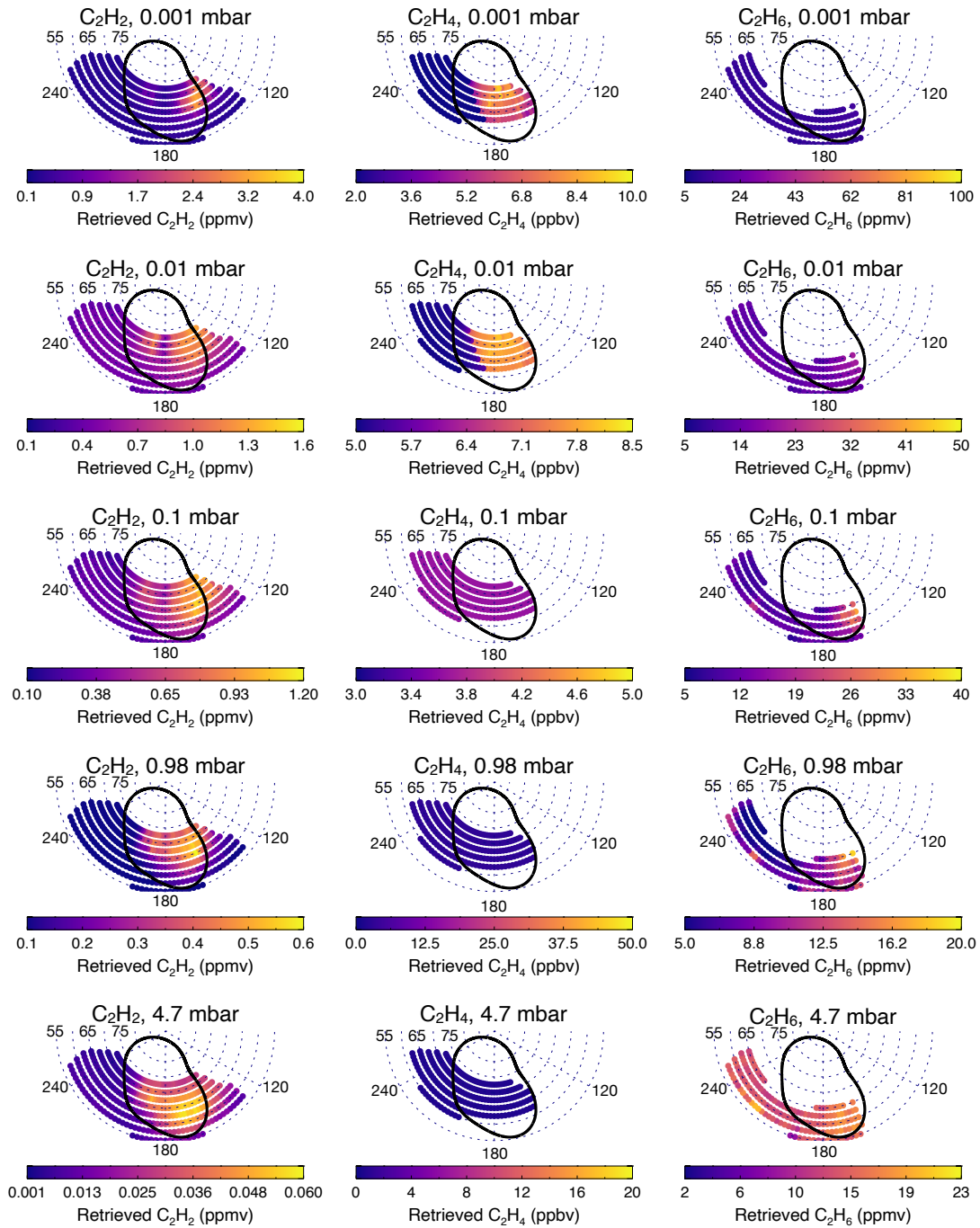
Figure 13. Retrieved abundances of C_2H_2 (left column), C_2H_4 (middle column) and C_2H_6 (right column) at high-southern latitudes on March 17th, 2017. Results are shown at 0.001 mbar (top row), 0.01 mbar (2nd row), 0.1 mbar (3rd row), 0.98 mbar (4th row) and 4.7 mbar (5th row). The solid, black line denotes the statistical-mean position of the ultraviolet auroral oval (Bonfond et al. 2017).
