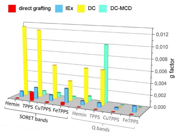
Figure 2. Maximum g factors on the Soret and Q bands for all the studied samples (nature of the porphyrins and nature of the interaction with the nanohelices)
