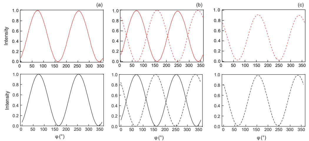
Figure 10. Transmitted intensity as a function of angle \varphi between the analyzer and the x -axis. The polarizer is along the x -axis and a quarter-wave plate has been inserted between the polarizer and the sample, with its slow axis at 45^\circ from the x -axis. Sample of thickness d = 6.05 μm. The curves on the top row are experimental and those in the bottom row are theoretical. From (a–c) V = 5, 6, and 6.3 Vrms. The solid line curves correspond to a TIC1 and the dashed lines to a TIC2. In (b) the curves in full line have been obtained by increasing the voltage and those in dashed line by decreasing the voltage.
