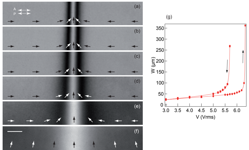
Figure 9. (a–e) Pi-wall between two TIC1 oriented in opposite directions which forms spontaneously in the middle of the 6.05 μm-thick sample when a voltage larger than V_{th} is applied. From (a–e) V = 3.5, 4, 5, 6, 6.3 Vrms. The wall is perpendicular to the magnetic field B . (f) TIC2 observed at V = 6.8 Vrms. The arrows indicate how the \vec{c} -director rotates in the sample. Observation without the quarter-wave plate between crossed polarizers (analyzer parallel to B ). The white bar is 50 μm long. (g) Width W of the pi-wall as a function of the voltage measured at increasing and decreasing voltage.
