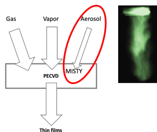
Fig. 1. Strategies for (multi)functional thin film plasma deposition. An image of aerosol taken by rapid imaging is reported inset.
