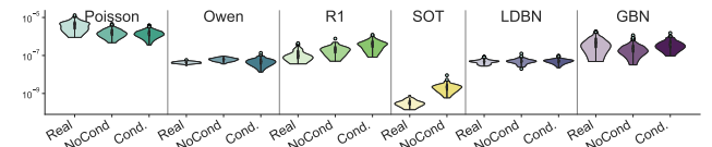
Figure 7: We compare the vanilla per class trained model with the global conditioned one for the integration error metric on Gaussian integrands for 1024 samples.
