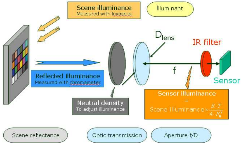
Figure 8: Measurement set-up
