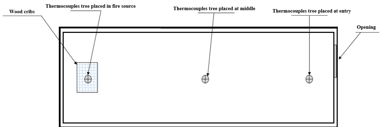
4b) Top view with the location of the fire origin
