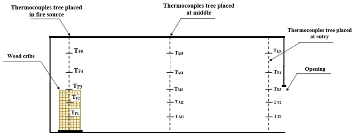
4a) Side view with arrangement of the thermocouples
