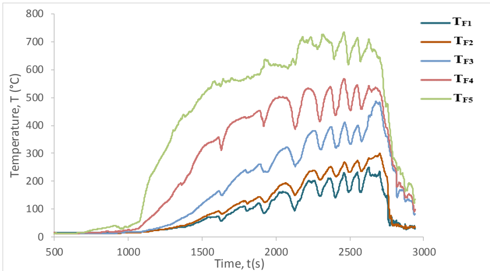
5a) at the fire origin
