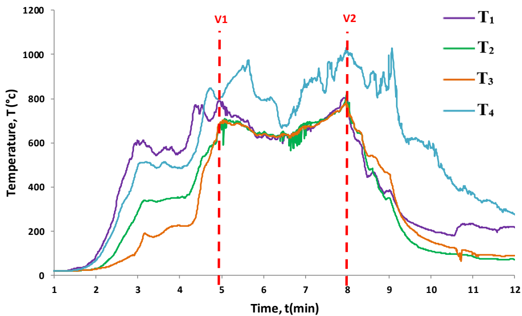
Figure 7. Evolution of the temperature during the test by applying two portable fans
