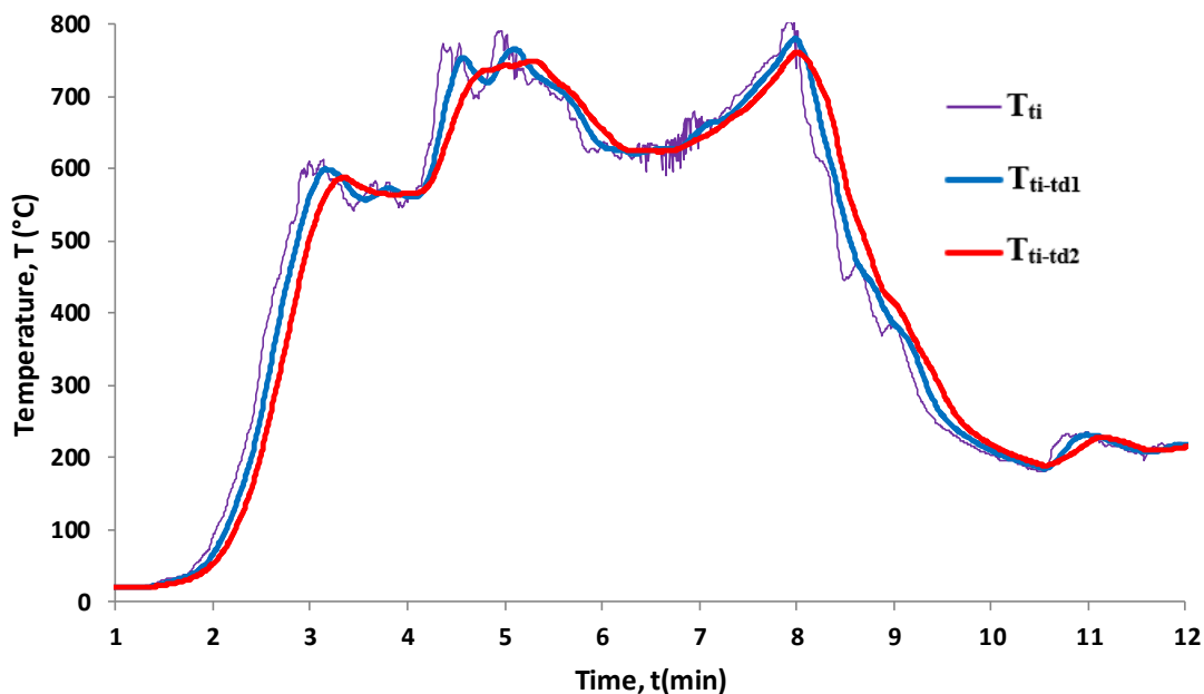
Figure 9. History of temperature inside the burning room and comparison of the two moving averages from the temperature ( T_1 ) recordings under the ceiling
