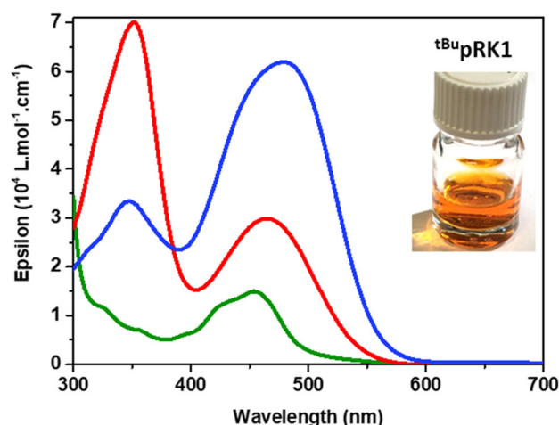
Figure 2. UV–vis absorption spectra of tBu_pRK1 (red line, recorded in DCM) and P1 (blue line, recorded in DCM), and RuP_2^{OEt-bpy} (green line, recorded in MeCN) and picture of a tBu_pRK1 solution.
