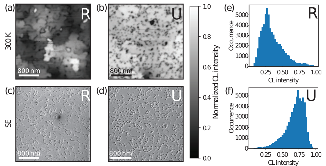
Figure 4. (a,b) show the panchromatic CL individually normalized integrated intensity images of 3.2 \times 3.2 \mu\text{m}^2 areas for samples R (a) and U (b), recorded at room temperature (groups of V-pits appear as large dark spots); (c,d) SE images for the same areas of each sample (R, U); V-shaped pits marking the position of TDs are visible as dark spots; (e,f) intensity histograms from the CL mappings.
