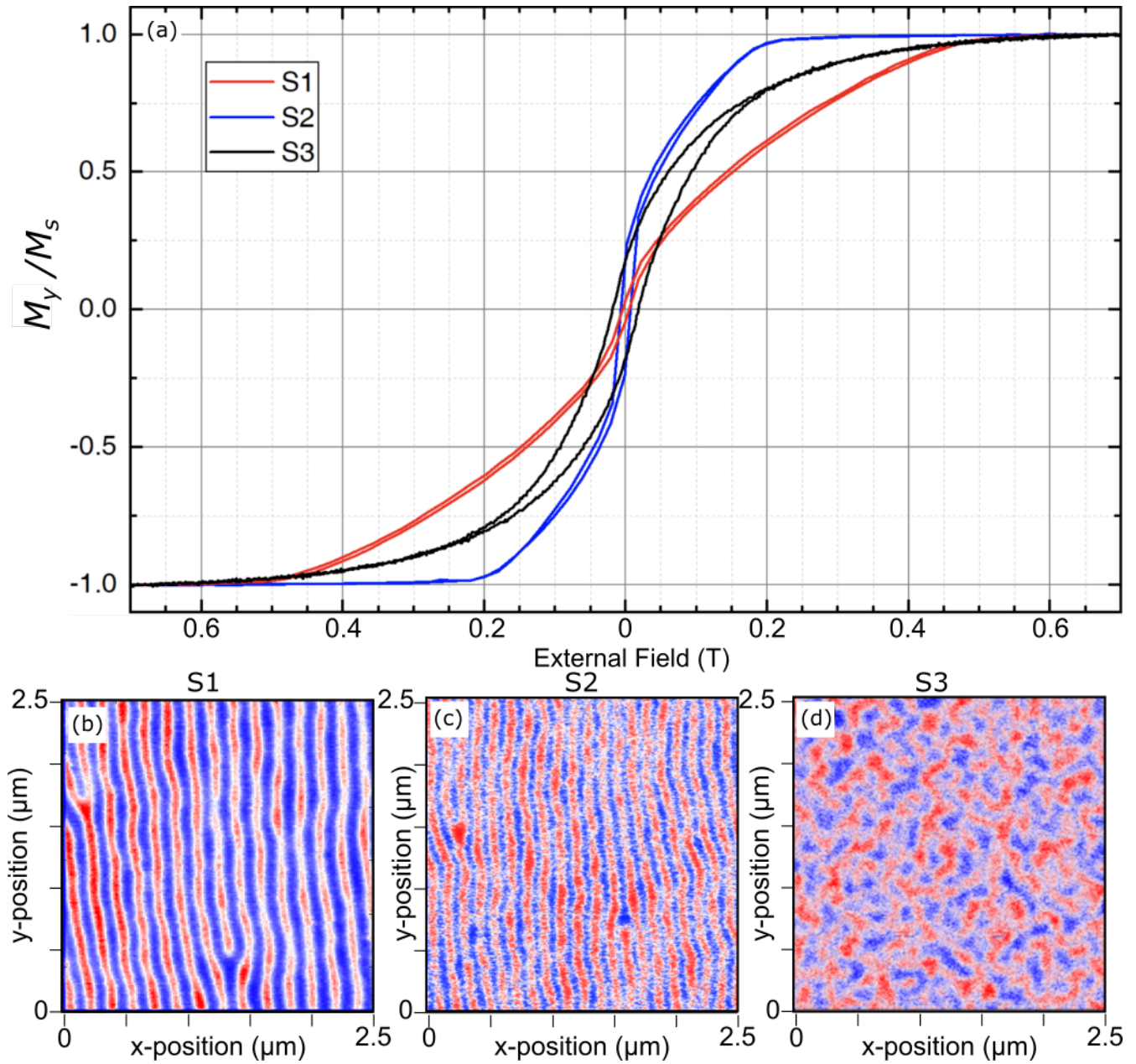
Figure 1. Magnetization hysteresis and zero-field MFM measurements for the three samples used in this work (sample details presented in the main text). (a) Hysteresis curves, normalized by the saturation magnetization M_s of each sample. (b-d) MFM phase maps for samples S1, S2 and S3 respectively. The colour codes the attraction of the magnetic tip (phase signal), and reveals the domain structure. The period is easily determined from such MFM images
