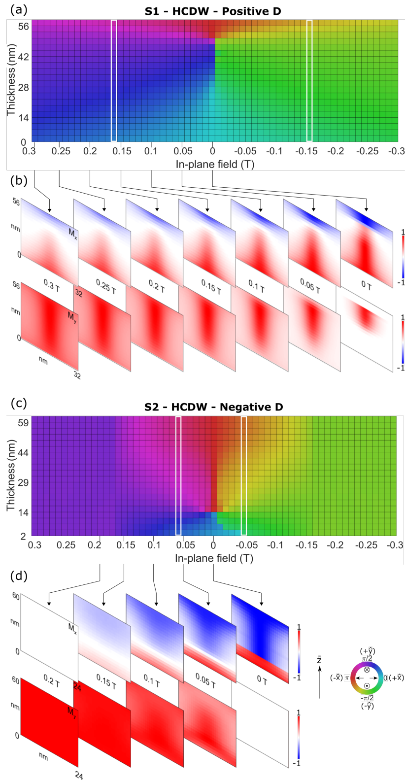
Figure 7. Azimuthal angle of the magnetization at each layer (rows) along the vertical direction (columns) of a single domain wall. Each column represents each field step between 0.3 to -0.3 T for sample (a) S1 and (c) S2. The angles were calculated using micromagnetic simulations. The direction of the in-plane magnetization associated to the colour scale is graphically displayed by the inner symbols of the colour wheel. White rectangles point the external in-plane field at which the top layer angle is at 45 degrees from pure Néel or pure Bloch texture. We plot only the magnetic layer's magnetization without considering the spacer and heavy metal layers. The (b) and (d) panels show snapshots of the M_x and M_y components of the magnetization at different fields for S1 and S2 respectively.
