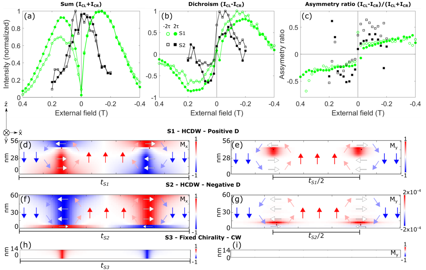
Figure 6. "Second order peak" intensity under an in-plane magnetic field. (a) The normalized sum, (b) normalized dichroism, and (c) asymmetry ratio of the left and right circular polarization XRRMS "second order peaks" ("SOPs") for sample S1 (green, circles), S2 (black, squares) respectively. Open (filled) represent the "SOP" at -2\tau ( +2\tau ). Data points are joined as a eyeguide. (d) - (i) Transversal cut along \hat{x} of micromagnetic simulations showing the \hat{x} and \hat{y} (background colour) and \hat{z} (arrows) components of the magnetization for S1 [(d), (e)], S2 [(f), (g)] and S3 [(h), (i)] respectively. We plot only the magnetization angle in the DW of each magnetic layer without considering the spacer and heavy metal layers. The colourbar in (g) has been modified to increase the contrast of M_y values for a better visualization. The magnetic states are shown at zero field after being saturated at 1 T in \hat{y} direction. Domain walls are spontaneously generated at random x position and are aligned for convenience. Points at 0 and 0.19 T are also shown in S. Flewett et al. 23 .
