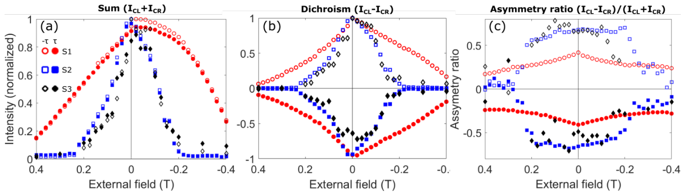
Figure 5. First order peak intensity under an in-plane magnetic field. (a) The normalized sum, (b) normalized dichroism, and (c) asymmetry ratio of the left and right circular polarization XMRS first order peaks (FOPs) for sample S1 (red, circles), S2 (blue squares) and S3 (black, diamonds) respectively. Open (filled) symbols represent the FOP intensity at -\tau ( +\tau ). In (a) - (c) the field scale is inverted to emphasize the temporal sequence from left to right.
