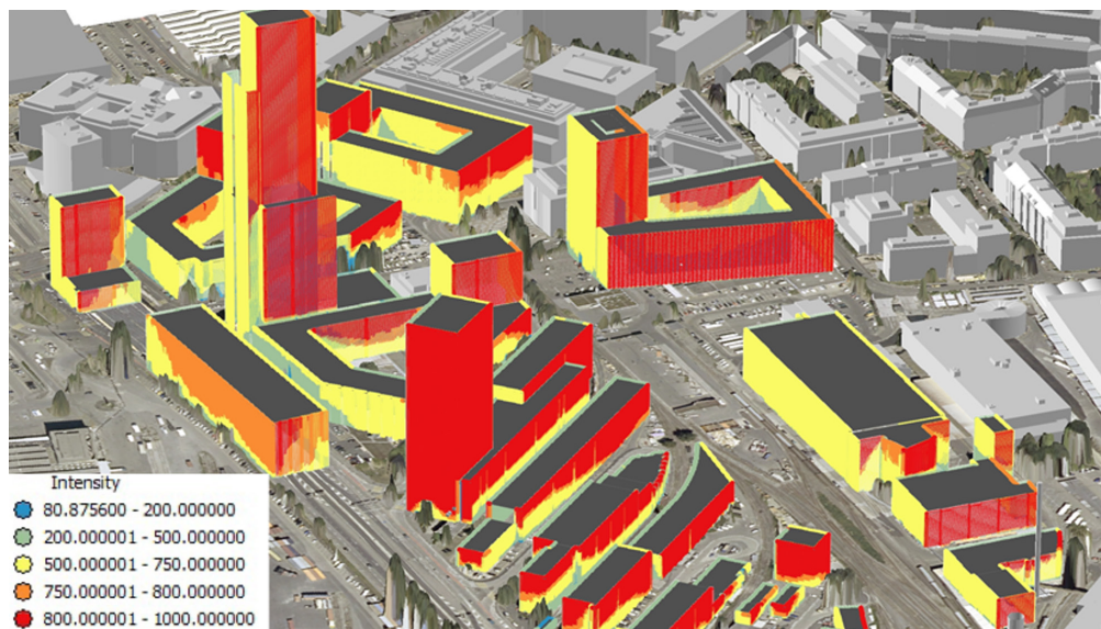
Simulation of solar radiation on facade on the new ND Grosselin in Carouge (Geneva)
