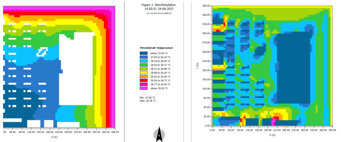
Simulation of project temperature and wind situation by ENVI-met
