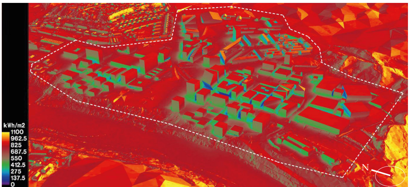
Annual irradiation analysis for feasibility study I.
