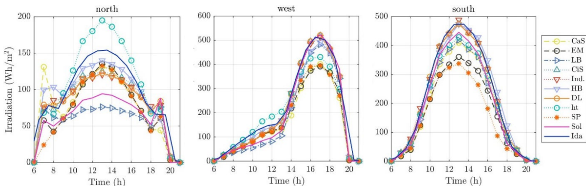
Figure 16: North, West and South façades for the unshaded case in February
