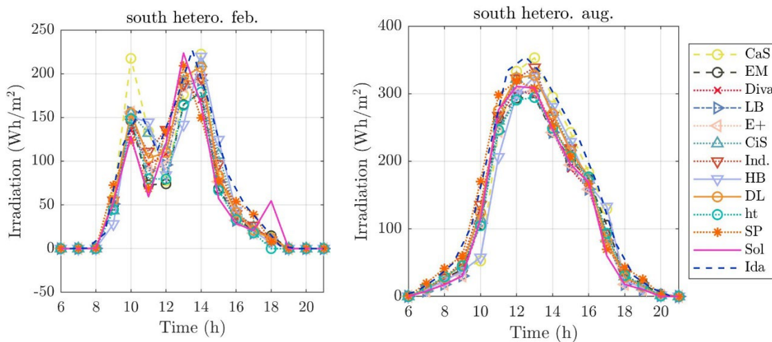
Figure 18 Irradiation on the southern face of the heterogeneous district (left) February, (right) August
