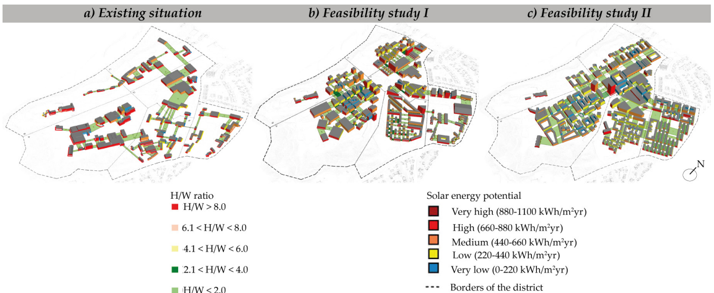
Solar potential of the facades depending on the H/W ratio (Feasibility Study I in the middle)
