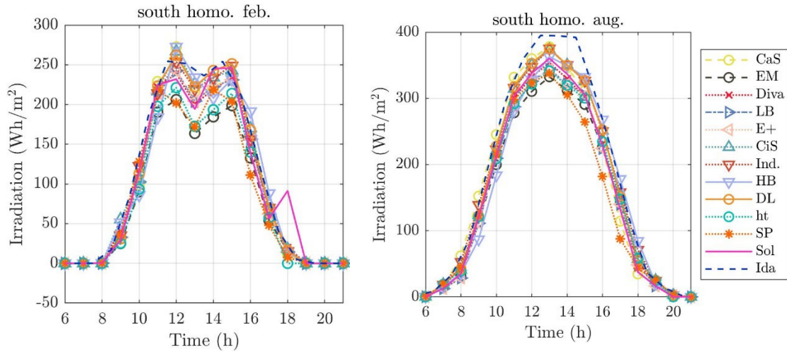
Figure 17: Irradiation on the southern face of the homogeneous district (left) February, (right) August
