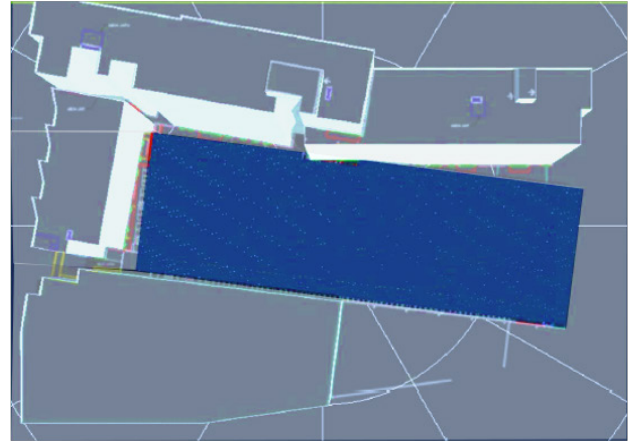
Distribution of PV on the roof of Building 23 (788 kWp) and parking (740 kWp). Source: s2e Technologies Inc.
