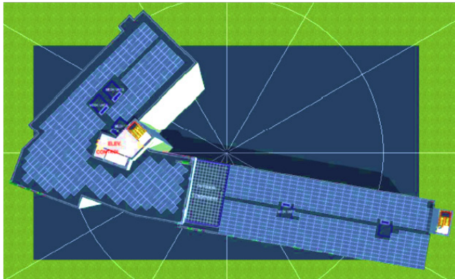
Distribution of PV on the roof of Building 19 (A) and south façade (B). Source: s2e Technologies Inc.
