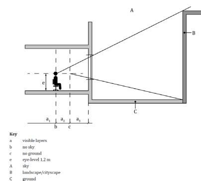
Figure C.6 — Cross-section for simplified verification method
