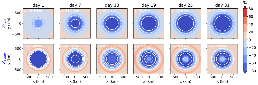
FIGURE 7 Horizontal cross-sections of PV anomaly (colours) and tracer mixing ratio (white contours: 0.1, 0.3, 0.5, 0.7, 0.9 \text{kg kg}^{-1} ) at the level of (top row) the tracer front Z_{front} and (bottom row) the tracer maximum Z_{center} , as follows from the reference (UP-REF) simulation.
