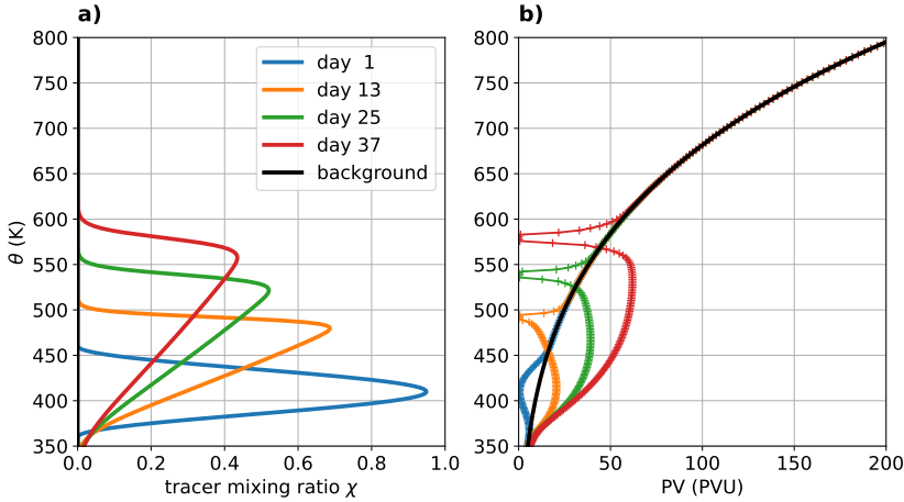
FIGURE 4 Numerical solution for the (a) tracer and (b) PV profile at the center of the structure ( R = 0 ). The parameters are \gamma = 5 \text{ K/day}/(\text{unit tracer mixing ratio}) , K_{\ominus} = 5 \text{ K}^2 \text{ day}^{-1} , and the initial condition is given by Equation (24). The background PV profile, shown in black in panel b, is typical for mid-latitudes (constant \bar{T} = 220 \text{ K} , f = 10^{-4} \text{ s}^{-1} ).
