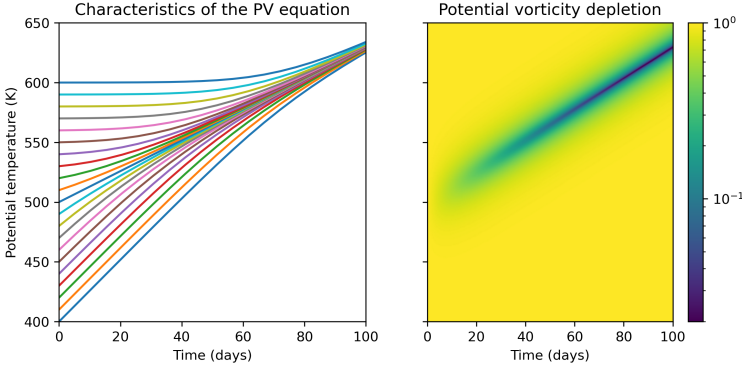
FIGURE A1 (a) Characteristic curves of the potential vorticity equation for \gamma = 5 \text{ K/day}/(\text{kg kg}^{-1}) , K = 17 \text{ K}^2/\text{day} , \chi_{max} = 1 and a front initially at \theta_0 = 500 \text{ K} . (b) Evolution of the potential vorticity ratio P/P_0 for these conditions.
