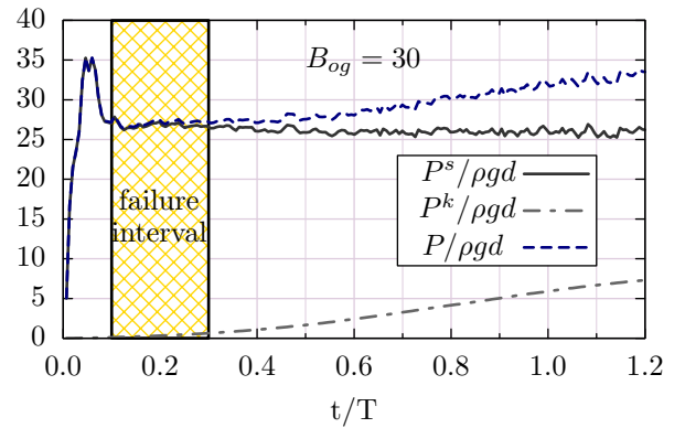
FIG. 8. Time evolution of pressure P^s , P^k and P computed from the static, kinetic and total stress tensors \sigma^s , \sigma^k and \sigma , here averaged on the simulation series with B_{og}=30 . The shaded area shows the failure time interval (see text).
