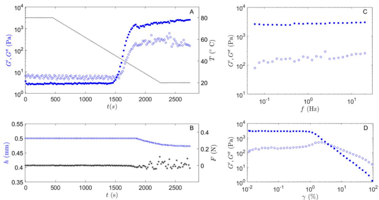
Figure 7. Rheological characterization of a gel sample ( [1\text{Br}_2] = 1.3 \text{ mM} , [\text{LiTFSI}] = 100 \text{ mM} , [\text{TBAI}] = 50 \text{ mM} in pentanol). A) Evolution of the viscous (hollow circles) and elastic (full blue squares) moduli in semilogarithmic scales determined through small-amplitude oscillations with \gamma = 0.1 \% and f = 1 \text{ Hz} during a cooling ramp of 2 \text{ }^\circ\text{C}/\text{min} ( T in black dots), (crossover temperature of G' and G'' : T_g = 44^\circ\text{C} ; terminal value of the elastic modulus: G' = 1700\text{-}2200 \text{ Pa} ; terminal value of the viscous modulus: G'' = 150\text{-}300 \text{ Pa} ). B) Evolution of the gap width h (blue crosses) while imposing a constant normal force F (black stars) during the cooling ramp (relative decrease of the gap width: \Delta h/h = 4.8 \% ). C) Frequency sweep experiment conducted between 20 \text{ Hz} and 0.06 \text{ Hz} on the freshly in-situ formed gel, 10 \text{ pts/decade} , \gamma = 0.05\% . D) Strain sweep experiment conducted for \gamma = 0.01\% up to 500\% on the freshly in-situ formed gel (yield strain value: \gamma_y = 4\% ).
