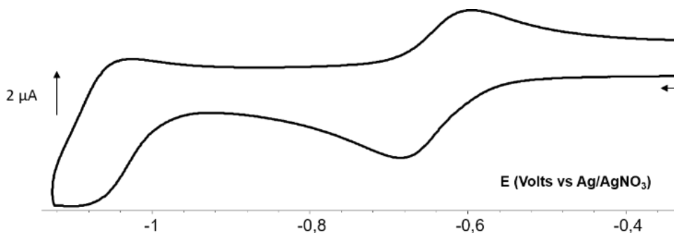
Figure 9. Cyclic voltammogram of the 1^{2+} gel in 1-pentanol ([TBAI]=50mM, [LiTFSI]=100mM, [1(\text{Br})_2] = 1.3\text{mM} ). Fresh gel formed around a Pt grid used as working electrode, v=10\text{mV/s} .
