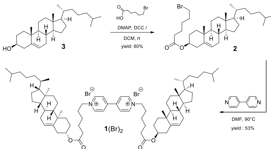
Scheme 1. Synthesis of 1(Br) 2 .
