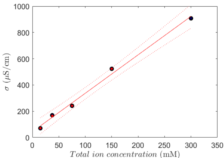
Figure 3. Evolution of the ionic conductivity with the total concentration in salts ( [\text{TFSI}^-]/[\text{I}^-] = 2 in all experiments). Black dots represent the ionic conductivity measured for gels obtained from the self-assembly of 1 (Br) 2 (0.2 wt% in pentanol). Red dots correspond to the ionic conductivity
