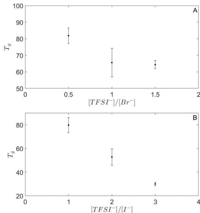
Figure 2. Influence of the concentration ratio between bistrifluoromethylsulfoniylimide (TFSI - ) and halide ions (I - or Br - ) on the gelation temperature ( T_g ) in pentanol. Each point corresponds to the mean value obtained for a series of rheological measurements. The error bars correspond to the standard deviations of each series. A) For all samples tested ( 1 (Br) 2 = 0.2 wt% = 1.3 mM in pentanol), the source of TFSI - anions was LiTFSI. B) For all samples tested [TFSI - ] = 100 mM, 1 (Br) 2 = 0.2 wt% = 1.3 mM in pentanol, the source of iodide anions was TBAI.
