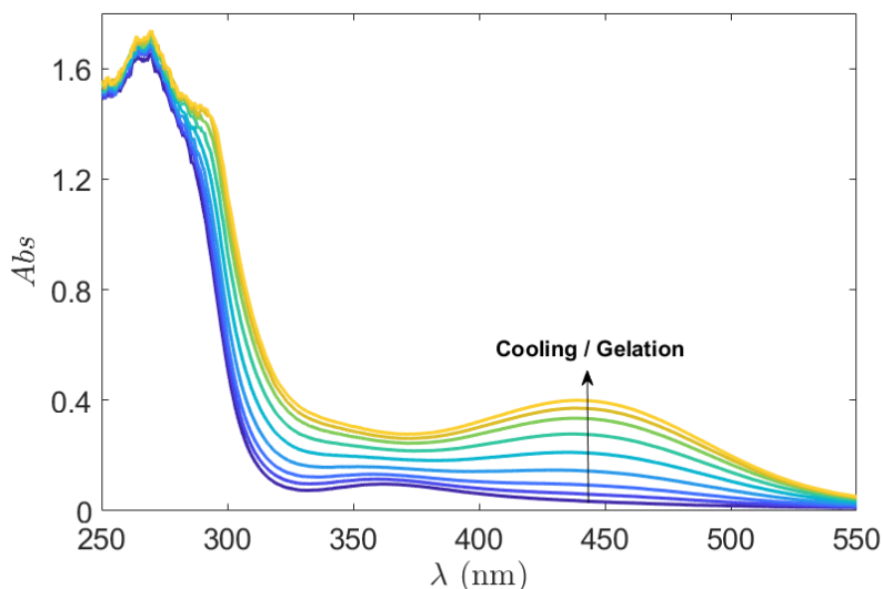
Figure 4. UV-vis absorbance spectra recorded over time during slow cooling of a hot solution of \mathbf{1}(\text{Br})_2/\text{LiTFSI}/\text{TBAI} in pentanol ( [\mathbf{1}(\text{Br})_2] = 1.3 \text{ mM} , [\text{LiTFSI}] = 100 \text{ mM} , [\text{TBAI}] = 50 \text{ mM} ) down to room temperature. Gelation of the sample upon cooling results in the development of a broad band at \lambda_{\text{max}} = 440 \text{ nm} .
