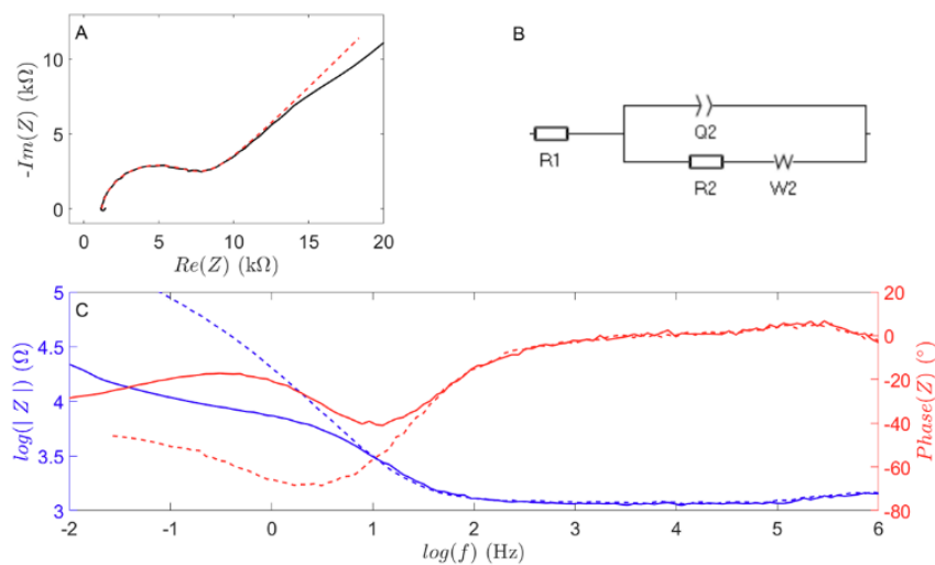
Figure 8. A) Black line: Nyquist plot of a gel sample ( [1^{2+}] = 1.3 \text{ mM} (0.2 wt%), [\text{LiTFSI}] = 100 \text{ mM} , [\text{TBAI}] = 50 \text{ mM} in pentanol). Red dashed lines: Nyquist plot corresponding to the equivalent circuit used to fit experimental data. B) Nyquist plot corresponding to the equivalent circuit used to fit experimental data ( R_1 = 1\,190 \text{ } \Omega , Q_2 = 8.804 \text{ } \mu\text{Fs}^{-0.104} , R_2 = 6\,074 \text{ } \Omega , W_2 = 2657
