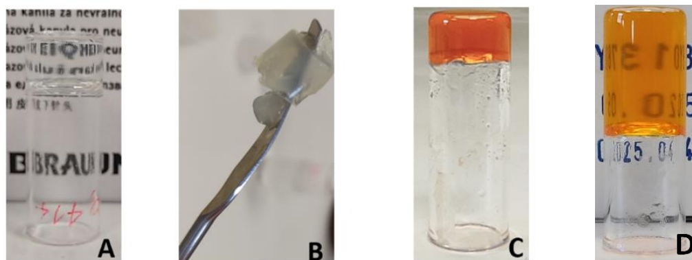
Figure 1. Pictures of gels obtained in different conditions. A) [1(\text{Br})_2] = 0.6 \text{ mM} (0.1 wt%) in BuOH. B) [1(\text{Br})_2] = 2.5 \text{ mM} (0.4 wt%), [\text{LiTFSI}] = 2.5 \text{ mM} in BuOH. C) [1(\text{Br})_2] = 2.5 \text{ mM} (0.4 wt%), [\text{TBAI}] = 0.1 \text{ M} in BuOH in presence of tetrabutylammonium iodide (TBAI). D) [1(\text{Br})_2] = 1.3 \text{ mM} (0.2 wt%), [\text{LiTFSI}] = 100 \text{ mM} , [\text{TBAI}] = 50 \text{ mM} in Pentanol. Vial diameter is ca. 1cm.
