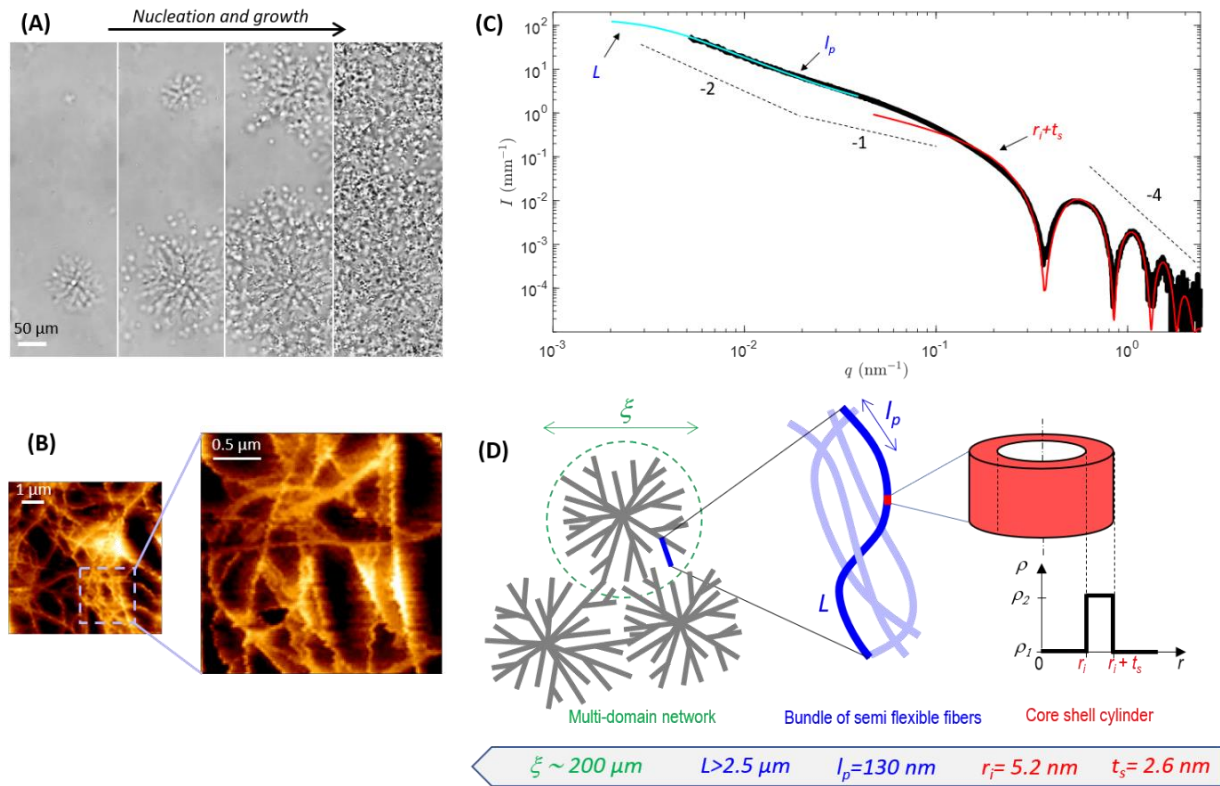
Figure 6. Determination of the gel structure using light microscopy, AFM, and SAXS. (A) Microscopy bright-field images of the sol-gel transition using a 15x magnification. The sol-gel transition proceeds through a nucleation and growth mechanism. (B) AFM images of the gel final state. (C) Scattering intensity I(q) of the gel final state as a function of the amplitude q of the scattering wave vector (black line) measured using SAXS. At low q , the blue line is the best fit of I(q) using an isotropic dispersion of flexible cylinders of persistence length l_p and length L (fitting range: 0.005 \text{ nm}^{-1} < q < 0.04 \text{ nm}^{-1} ). We obtain l_p = 130 \text{ nm} and L = 2.5 \mu\text{m} . Due to the limited range at low- q , L = 2.5 \mu\text{m} is the smallest filament length for which the fit works. The filaments have therefore a length, L > 2.5 \mu\text{m} . At large q , the red line is the best fit of I(q) using an isotropic
