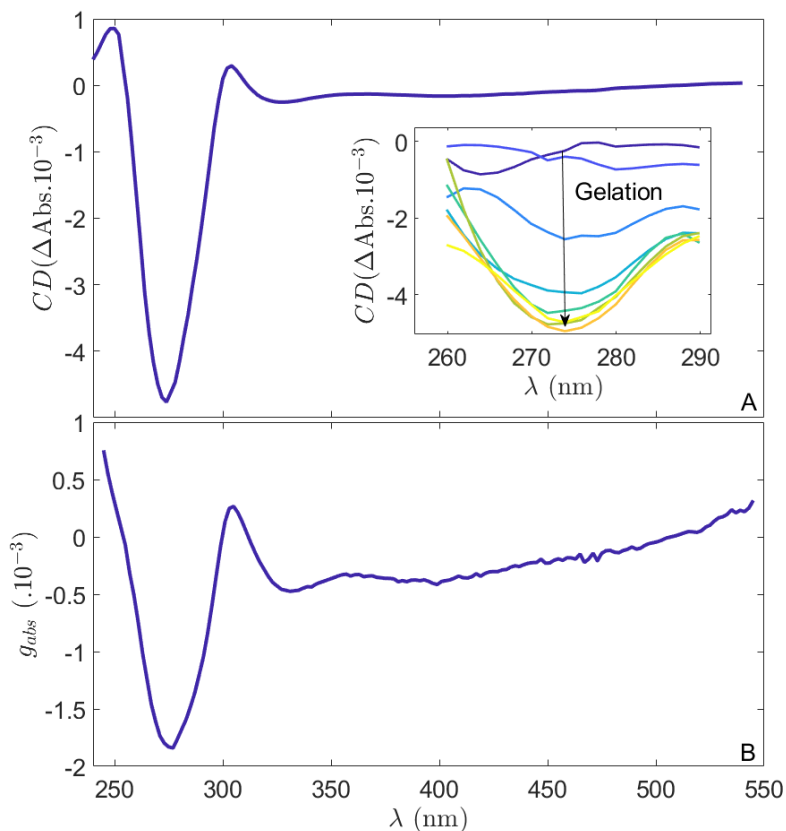
Figure 5. A) Electronic circular dichroism spectra collected for gels of \mathbf{1}^{2+} obtained in pentanol ( [\mathbf{1}(\text{Br})_2] = 1.3 mM, [\text{TBAI}] = 50 mM, [\text{LiTFSI}] = 100 mM). The inset shows the evolution of the CD signal after heating the gel above T_g and then leaving it cooling down to room temperature. B) g_{\text{abs}} spectra collected for gels of \mathbf{1}^{2+} obtained in pentanol ( [\mathbf{1}(\text{Br})_2] = 1.3 mM, [\text{TBAI}] = 50 mM, [\text{LiTFSI}] = 100 mM).
