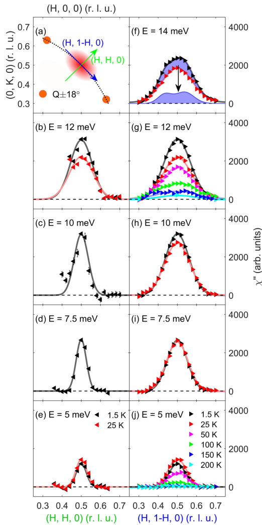
FIG. 2. (a) Schematic diagram of longitudinal and transverse scan. Q \pm 18^\circ marked in the Brillouin zone are measured by rotating the sample by \pm 18^\circ and used to subtract the nonmagnetic background. (See Fig. S1 in the Supplemental Material.) (b)–(e) Longitudinal Q scans of the imaginary part of the magnetic susceptibility \chi''(\mathbf{Q}, \omega) at various energy transfers in the normal state at T = 25 K (red triangle) and the superconducting state at T = 1.5 K (black triangle). (f)–(j) Transverse Q scans of the imaginary part of the magnetic susceptibility \chi''(\mathbf{Q}, \omega) at various energy transfers and temperatures. The solid lines are fitted by a Gaussian function except for the Q scan at T = 1.5 K and E = 14 meV (f) which is fitted by summing a Gaussian function ( Q scan at T = 25 K and E = 14 meV) and two symmetric Gaussian peaks. The double-peak structure of the Q scan at T = 1.5 K and E = 14 meV (f) can be clearly shown in the blue shaded area with a flat background. The background was estimated by the Q scans. (See Figs. S2 and S3 in the Supplemental Material [25].)
