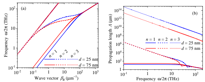
FIG. 2: Spectra of the in-plane (a) wave vector and (b) propagation length of the 3 SPP modes propagating along a graphene-coated Si film with d = 25 and 75 nm.
