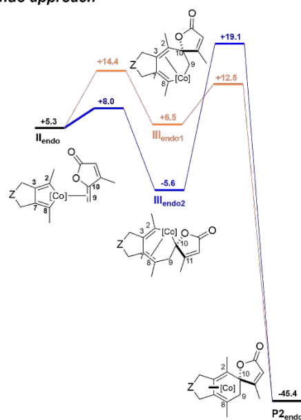
Figure 3. Computed exo - and endo - pathways. Z=C(CO 2 Me) 2 , [Co]=CpCo. \Delta G are computed at the TPSS-D3/def2-TZVP level (T=383.15K). Solvent effects are added as single point calculations with the COSMO implicit model (toluene).
