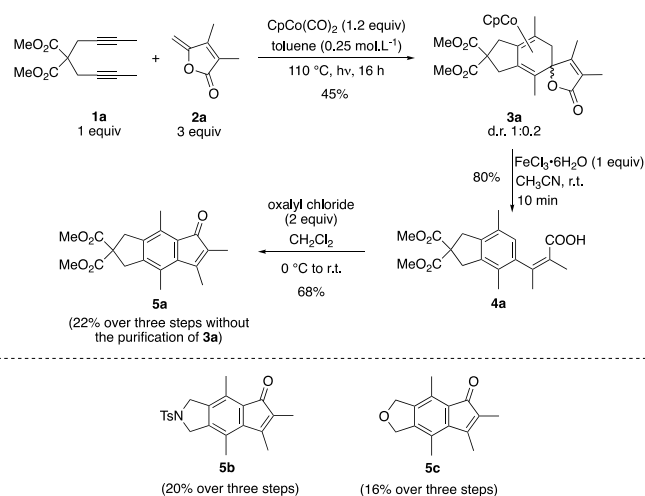
Scheme 2. Experimental evidence and post-functionalisation.
