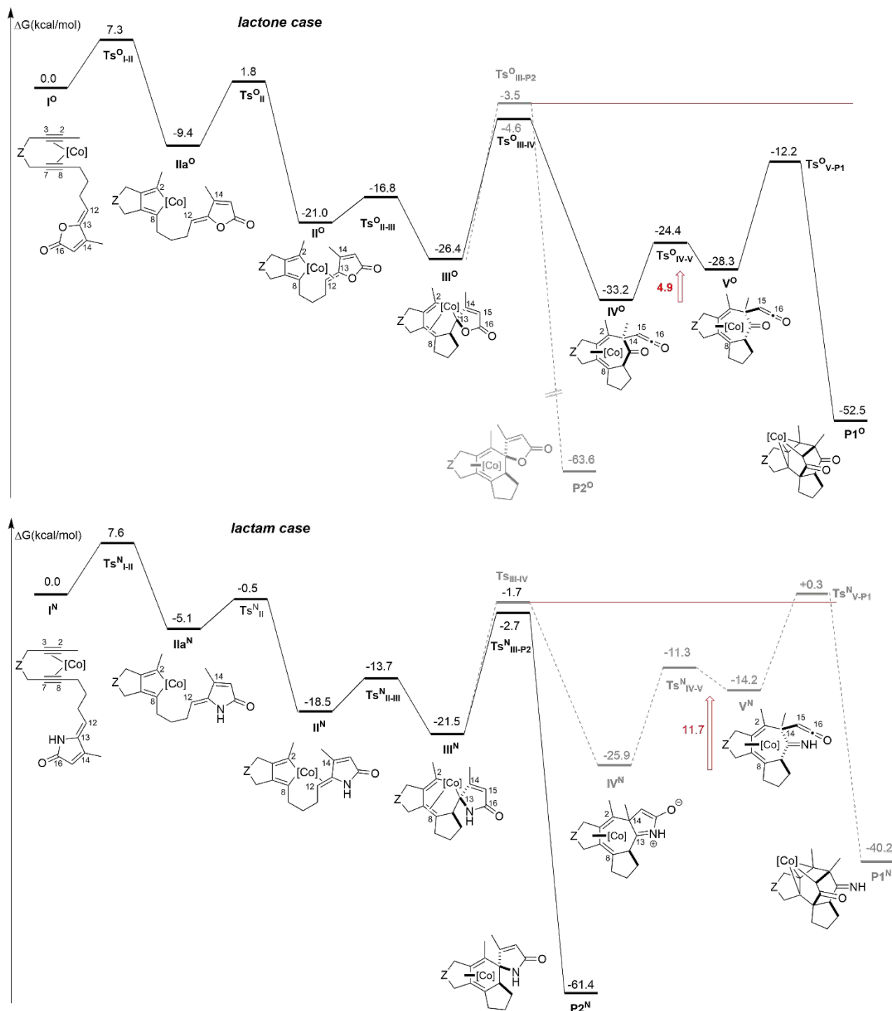
Figure 5. Computed pathways for the possible intramolecular reactions. On top, lactone case, and lactam case at the bottom, Z=C(C(O)OMe)_2 , [Co]=CpCo . \Delta G are computed at the TPSS-D3/def2-TZVP level ( T=383.15K ). Solvent effects are added as single point calculations with the COSMO implicit model (toluene).
