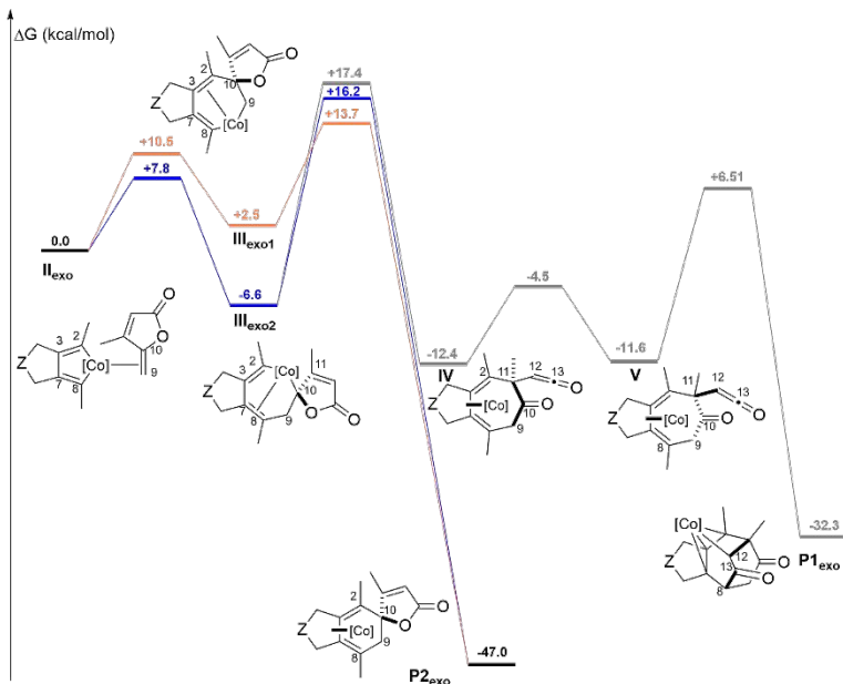
Figure 3. Computed exo - and endo - pathways. Z=C(CO 2 Me) 2 , [Co]=CpCo. \Delta G are computed at the TPSS-D3/def2-TZVP level (T=383.15K). Solvent effects are added as single point calculations with the COSMO implicit model (toluene).
