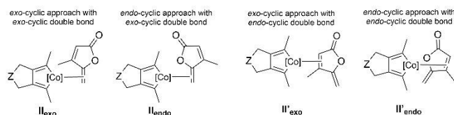
Figure 2. Different coordination modes for the intermolecular approach.
