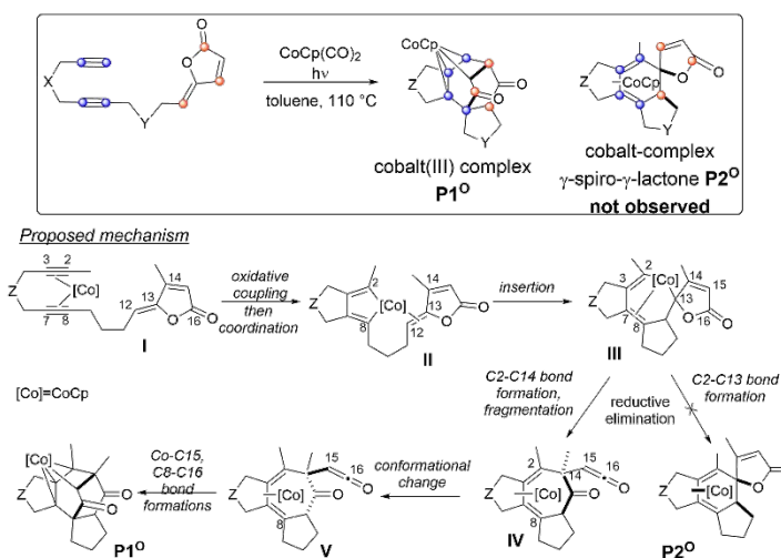
Scheme 1. Proposed mechanism for the cobalt-mediated formal (2+2+3) reaction.
