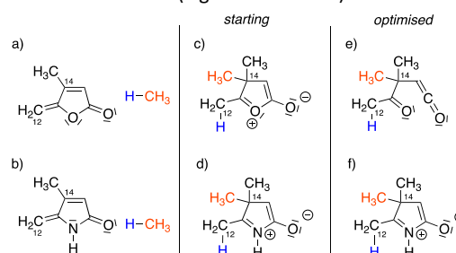
Figure 4. Model reactivity. 'Starting' denotes the initial structures and 'Optimised' denotes the structure obtained after the geometry optimisations (PBE0/def2-TZVP).
