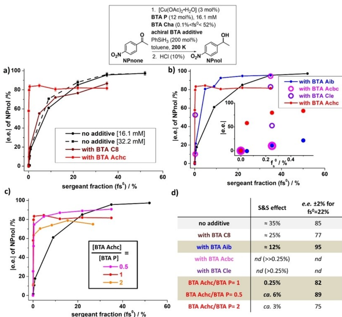
Figure 2. Catalytic evaluation of the effect of achiral BTA additives under the conditions indicated above the figure (conversion >99\% in all cases). All e.e. values are plotted in Tables S1–S3. a) Plot of the e.e. in NPnol as a function of f_s^0 for the S&S-type mixtures without achiral BTA additive and with BTA C8 or BTA Achc ( [\text{achiral BTA}]/[\text{BTA P}] = 1 ). b) Plot of the e.e. in NPnol as a function of f_s^0 for the S&S-type mixtures embedding the different achiral BTA additives ( [\text{achiral BTA}]/[\text{BTA P}] = 1 ). The plot for the mixture without additive (black) is shown for comparison. For BTA Acbc and BTA Cle, only a few catalytic mixtures have been evaluated that correspond to very low ( f_s^0 = 0.25\% ) or high ( f_s^0 = 35\% ) “sergeant” contents. Inset: zoom to distinguish the effect of achiral BTA additives at low f_s^0 values. c) Plot of the e.e. in NPnol as a function of f_s^0 for the S&S-type mixtures with different ratios of BTA Achc over BTA P. d) Table indicating the extent of the S&S effect and the enantioselectivity in NPnol (for f_s^0 = 22\% ) for the mixtures with and without additives. nd: not determined.
