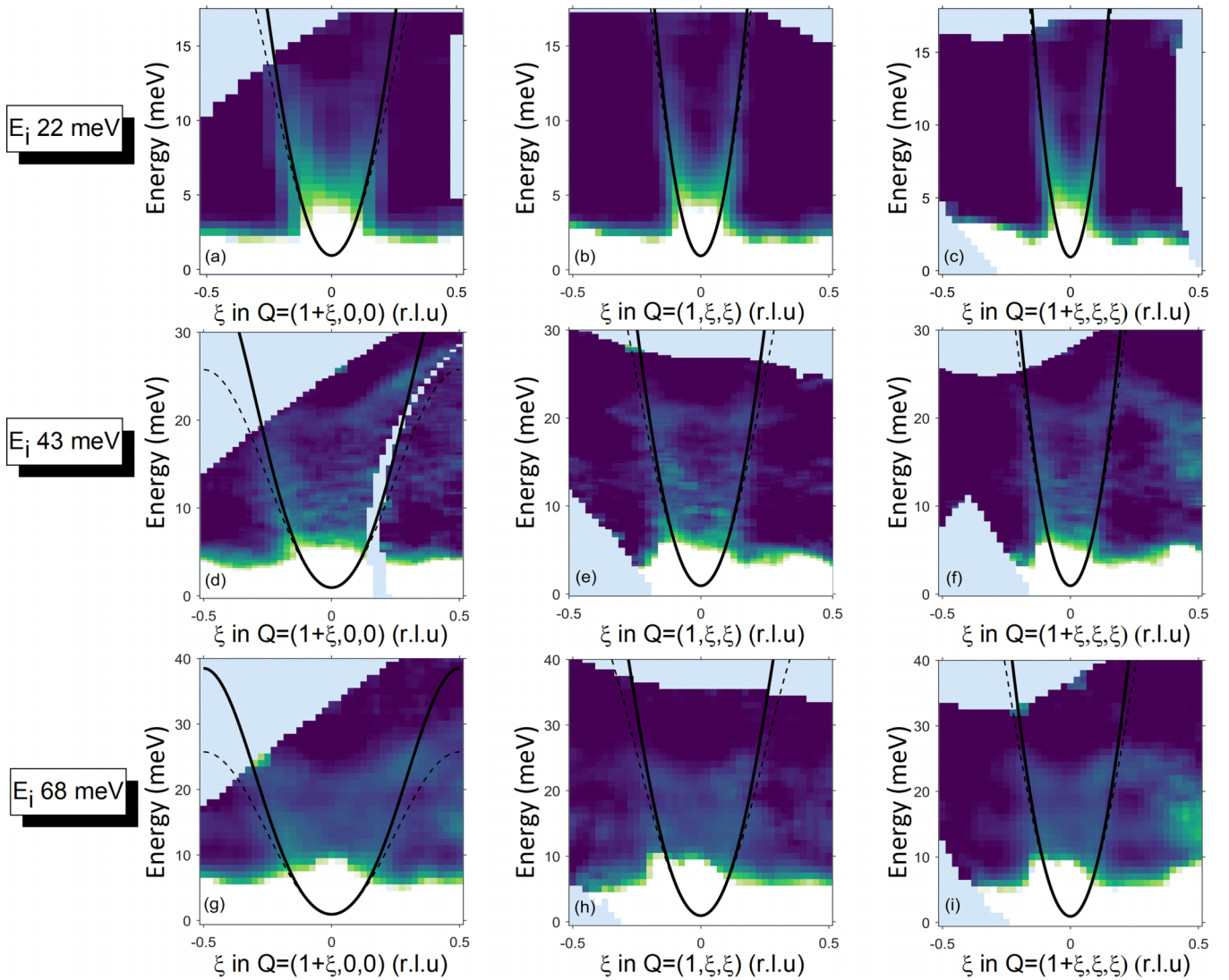
FIG. 6. Magnon dispersion measured by time-of-flight technique. Constant \mathbf{Q} cuts at 10 K along the cubic high-symmetry directions around \mathbf{Q} = (1,0,0) show the magnon dispersion. The panels are sorted in rows where each row represents the data of a certain incident energy. From the top to the bottom, the data are taken with 22 [(a)–(c)], 43 [(d)–(f)], and 68 meV [(g)–(i)], respectively. The intensity range (color bar) is set identical in the panels of each row for better comparability. The integration limits are -0.1 \leq \eta \leq 0.1 in [1, -\eta, \eta] and -0.1 \leq \zeta \leq 0.1 in the direction perpendicular to the respective high-symmetry direction. The time-of-flight data are overlaid with the ferromagnetic dispersion model with nearest-neighbor interaction J_1 (dashed line) and with the combination of nearest-neighbor and J_4 interaction (black lines).
