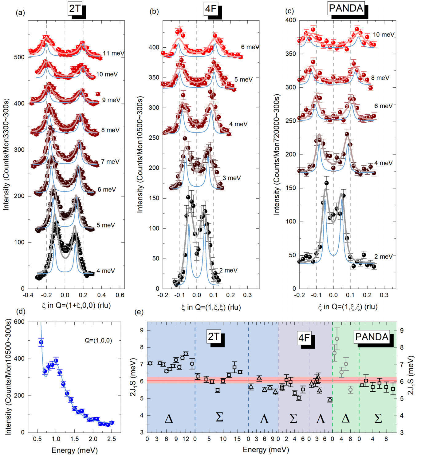
FIG. 2. (a)–(c) Constant energy scans across the magnon dispersion in SrRuO 3 obtained at T = 10 K on cold triple-axis spectrometers 4F (LLB) and PANDA (MLZ), and on the thermal spectrometer 2T (LLB). Note that the PANDA data were measured after detwinning the sample with magnetic field. The magnon scattering was modeled following the ferromagnetic dispersion relation including energy broadening (light blue lines) and then folded with the \mathbf{Q} and E dependent resolution function (colored lines). Data are vertically offset for clarity. (d) Constant \mathbf{Q} scan at \mathbf{Q} = (1, 0, 0) described with the same dispersion relation showing the anisotropy gap at T = 10 K (data taken on 4F). (e) The fitting yields a value of 2J_1S for each scan along different high symmetry directions. The data are distinguishable by colored background in respect to the instrument and by symbol shape in respect to the cubic direction (circle: \Delta = [\xi, 0, 0] ; square: \Sigma = [0, \xi, \xi] ; triangle: \Lambda = [\xi, \xi, \xi] ). The weighted average of 2J_1S = 6.1(2) meV is represented by the red line while the light red area denotes its error margin. Data in gray are not used for the averaging. Data in panels (a) and (b) were already presented in Ref. [25].
