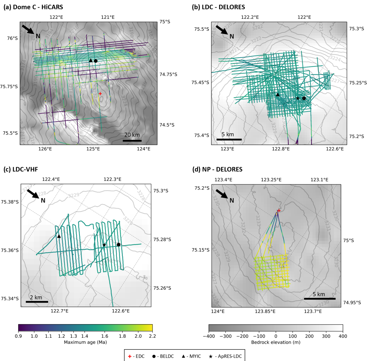
Figure 11. Maximum age with a maximum acceptable age density of 20 \text{ kyr m}^{-1} , colour bars correspond to all four panels. (a) HiCARS airborne dataset, (b) LDC DELORES ground-based dataset, (c) LDC-VHF high resolution ground-based dataset and (d) NP DELORES ground-based dataset.
