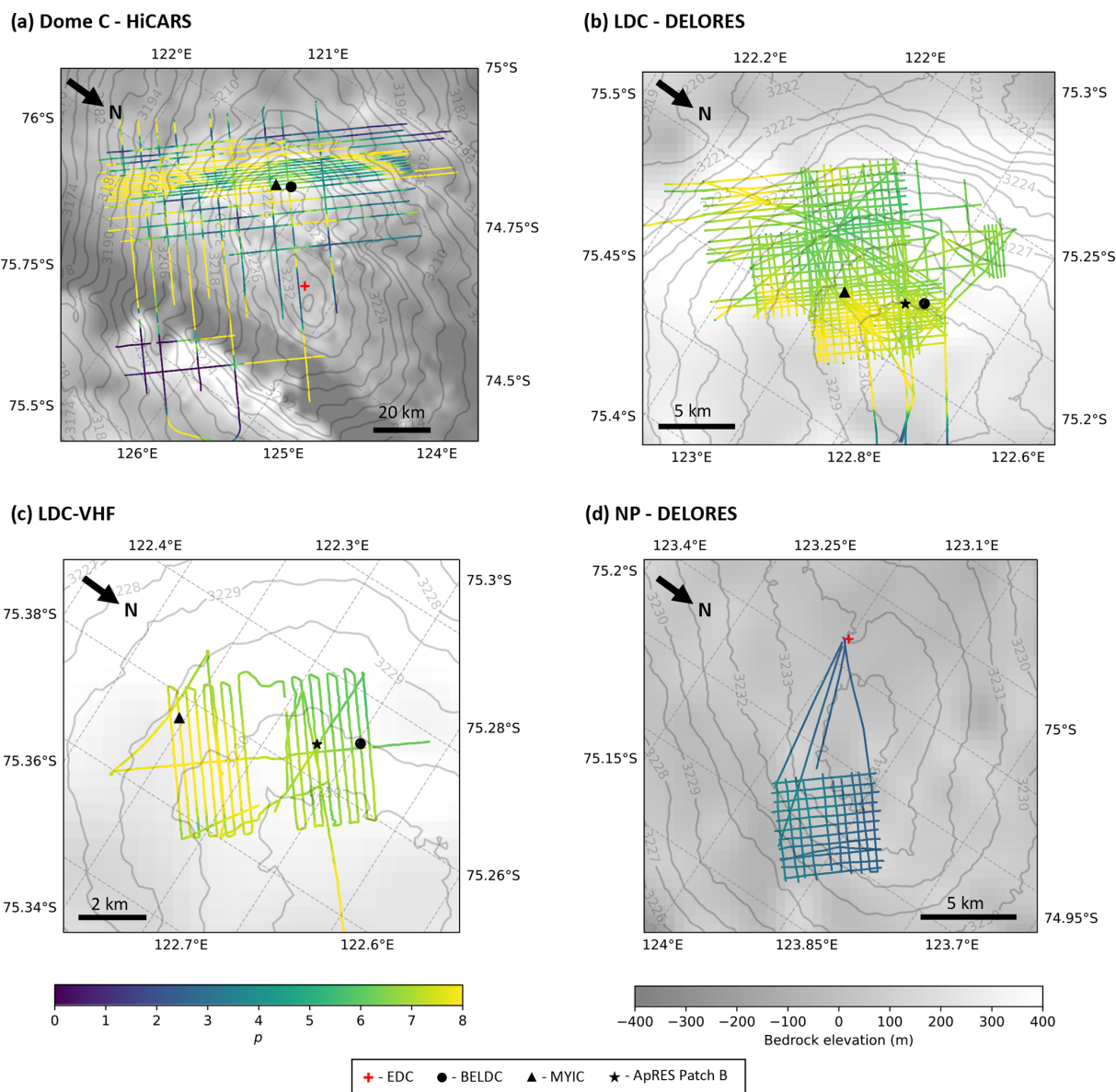
Figure 10. Llibouty profile p parameter, colour bars correspond to all four panels. (a) HiCARS airborne dataset, (b) LDC DELORES ground-based dataset, (c) LDC-VHF high resolution ground-based dataset and (d) NP DELORES ground-based dataset.
