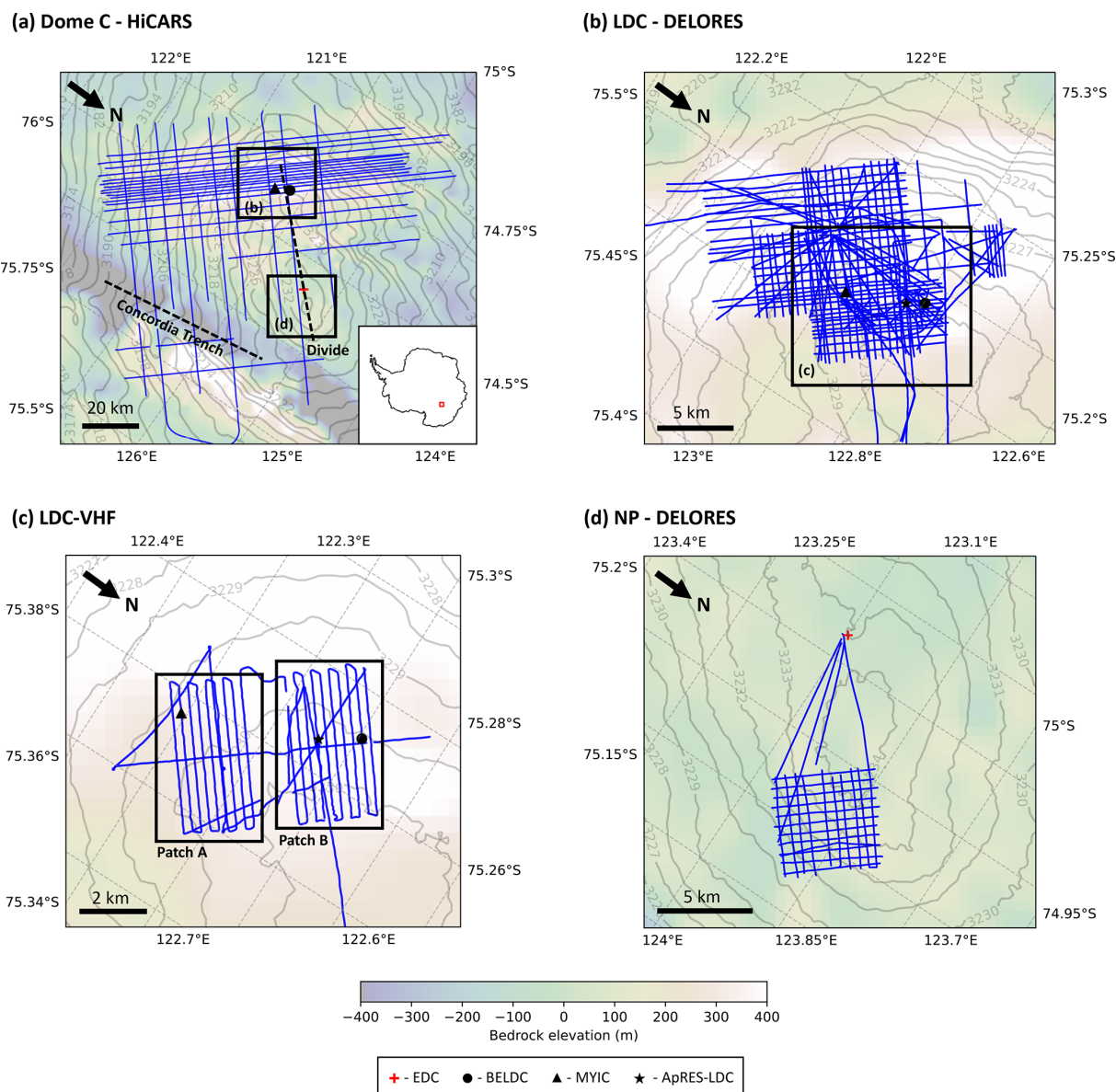
Figure 2. Maps showing the four areas of interest near Dome C, with bedrock elevation from BedMachine version 3 (Morlighem, 2022) and surface elevation from REMA (Howat et al., 2019). Radar transects of each survey are in blue. Ice core drill sites EDC, BELDC, MYIC and the ApRES-LDC site are marked by a red cross, black circle, black triangle and black star, respectively. (a) The larger Dome C region covered by the HiCARS airborne radar transects. The dashed black lines show the Concordia trench and Dome C divide. In the inset, the red square shows the location of Dome C in Antarctica. (b) LDC DELORES ground-based radar dataset, (c) LDC-VHF high resolution ground-based radar dataset and (d) NP DELORES ground-based dataset.
