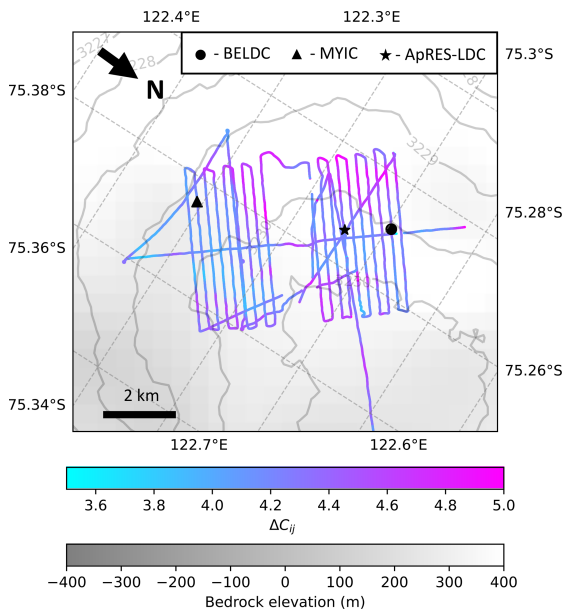
Figure 5. The \Delta C_{ij} value which compares the relevance of the model, which inverts H_m and the model, and which uses H_{obs} as a constraint, applied to the LDC-VHF radar dataset.
