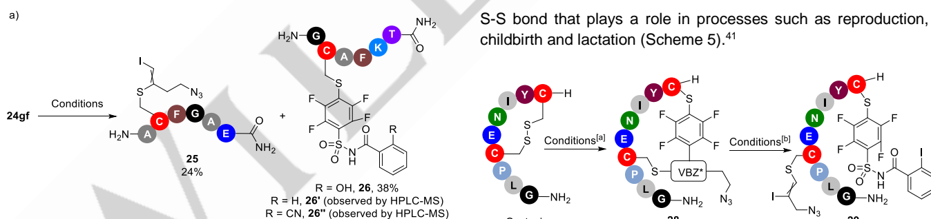
Scheme 4. Reaction conditions: 0.0025 mmol 24af , 0.025 mmol L-proline, 0.050 mmol CuCN, ACN : PB (50 mM, pH = 8.0) = 1 : 1, 2.5 mM with respect to 24gf , at 37 °C for 18 hours; isolated yields.
