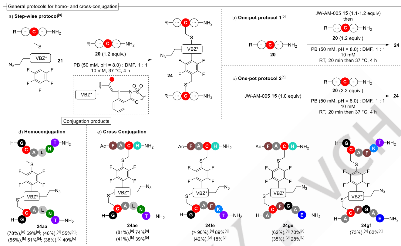
Scheme 3. [a] 0.0040 mmol 21 , 0.0044-0.0048 mmol 15 , PB (50 mM, pH = 8.0) : DMF, 1 : 1, 10 mM with respect to 21 , at 37 °C; (indicative HPLC-MS-based yields are reported in parentheses), isolated yields. [b] 0.0040 mmol 20 , 0.0048 mmol 15 , PB (50 mM, pH = 8.0) : DMF, 1 : 1, 10 mM with respect to 20 at room temperature for 20 minutes; then 0.0044-0.0048 mmol 20 at 37 °C; (indicative HPLC-MS-based yields are reported in parentheses), isolated yields. [c] 0.0072 mmol 20 , 0.0032 mmol 15 , PB (5.0 mM, pH = 8.0) : DMF, 1 : 1, 10 mM with respect to 20 , at 37 °C; (indicative HPLC-MS-based yields are reported in parentheses), isolated yield. [d] Same conditions as in [a] but at room temperature.
