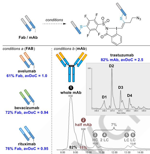
Scheme 6. Reaction conditions: [a] Fab (1.5 mg/mL in BBS, 2 mM EDTA, pH 8), TCEP (15 mM in water, 5 equiv.), 15 (10 mM solution in DMSO, 5 equiv.) at 37 °C for 5 hours. [b] trastuzumab (10 mg/mL in BBS, 6 mM EDTA, pH 8), TCEP (15 mM in H 2 O, 10 equiv.), 15 (10 mM solution in DMSO, 10 equiv.) at 37 °C for 5 hours. Chromatogram and mass spectrum excerpts from the dSEC-MS analysis of the rebridging of trastuzumab are provided.
