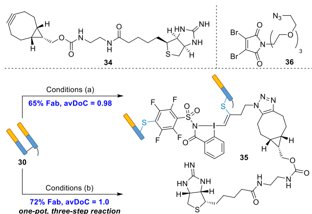
Scheme 7. Reactions conditions: [a] 1. Fab 30 (1.5 mg/mL in BBS, 2 mM EDTA, pH 8), TCEP (15 mM in water, 5 equiv.) 15 (10 mM solution in DMSO, 5 equiv.) at 37 °C for 5 hours; 2. 34 (10 mM in DMSO, 30 equiv.) at 25 °C for 24 hours. [b] Fab 30 (1.5 mg/mL in BBS, 2 mM EDTA, pH 8), TCEP (15 mM in H 2 O, 5 equiv.), 15 (10 mM solution in DMSO, 5 equiv.), 34 (10 mM solution in DMSO, 20 equiv.) at 37 °C for 5 hours.
