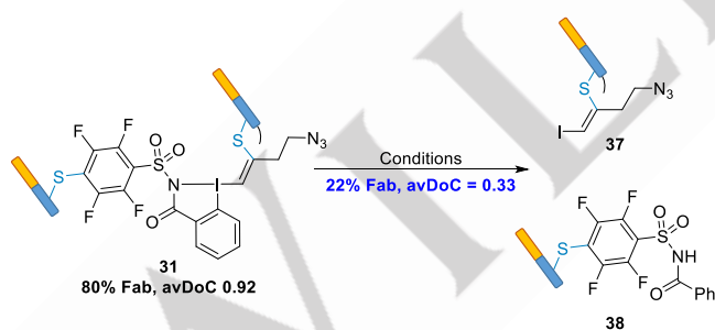
Scheme 8. Reaction conditions: 31 (1.5 mg/mL in PBS 1X, pH 7.4), 20 equiv. CuI, 40 equiv. THPTA, 100 equiv., aminoguanidine•HCl, 300 equiv. NaAsc, at 37 °C for 16 hours.
