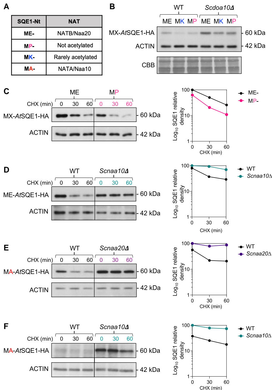
Figure 6. Impact of N-terminal mutagenesis on AtSQE1 stability suggests indirect effects of Nt-acetyltransferases on protein turnover in yeast. A ) Summary of N-terminal (Nt) mutants and predicted respective NAT activities. B ) Steady-state protein levels of AtSQE1-HA Nt-variants in WT and Scdoa10Δ yeast cells. C ) Cycloheximide (CHX) chase of WT ME- and mutant MP-AtSQE1-HA in WT yeast cells (immunoblot and quantified relative density). D ) Cycloheximide (CHX) chase of WT ME-AtSQE1-HA in WT and Scnaa10Δ yeast cells (immunoblot and quantified relative density). E ) Cycloheximide (CHX) chase of mutant MA-AtSQE1-HA in WT and Scnaa20Δ yeast cells (immunoblot and quantified relative density). F ) Cycloheximide (CHX) chase of mutant MA-AtSQE1-HA in WT and Scnaa10Δ yeast cells (immunoblot and quantified relative density).
