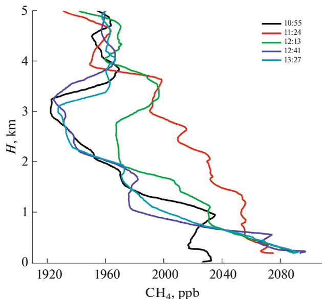
Fig. 4. Vertical distribution of the methane concentration over Naryan-Mar (10:55) and the Kara Sea (11:24, 12:13, 12:41, and 13:27), September 6, 2020.
