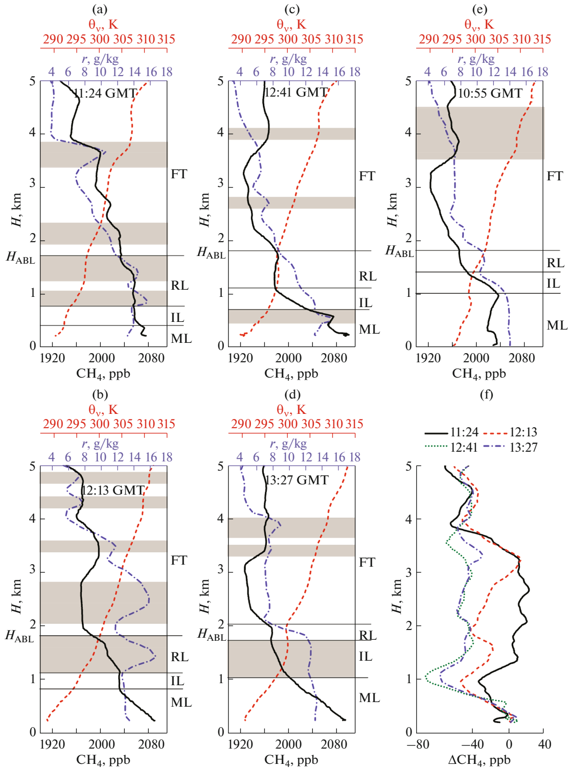
Fig. 5. Vertical distributions of the methane concentration (black curve), mixing ratio (blue curve), and virtual potential temperature (red curve) over (a–d) the Kara Sea and (e) in the Naryan-Mar region; (f) (land–sea) differences in methane concentrations on September 6, 2020.
