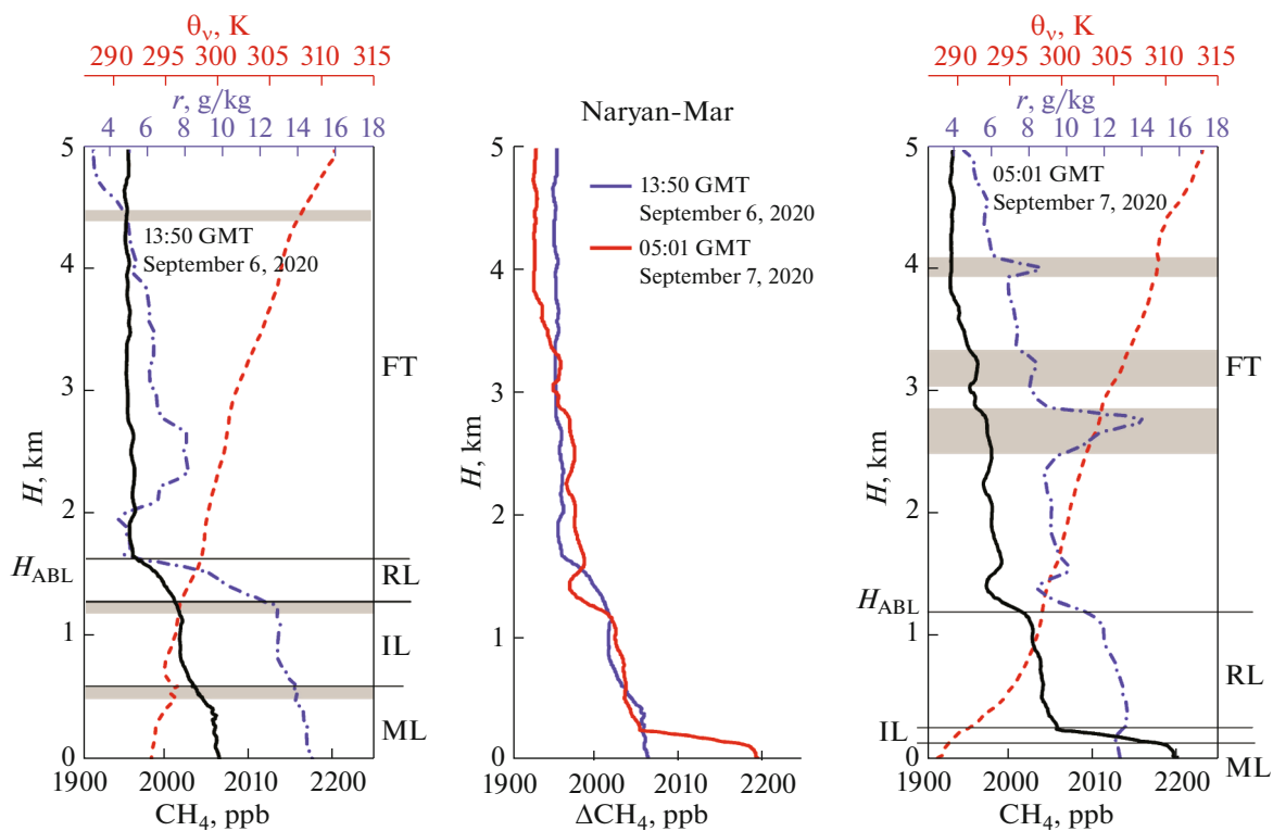
Fig. 17. (b) Vertical profiles of the methane concentration obtained in the Naryan-Mar region: (a, c) methane concentrations (black curve), mixture ratio (blue curve), and virtual potential temperature (red curve) on September 6 and 7, 2020.
