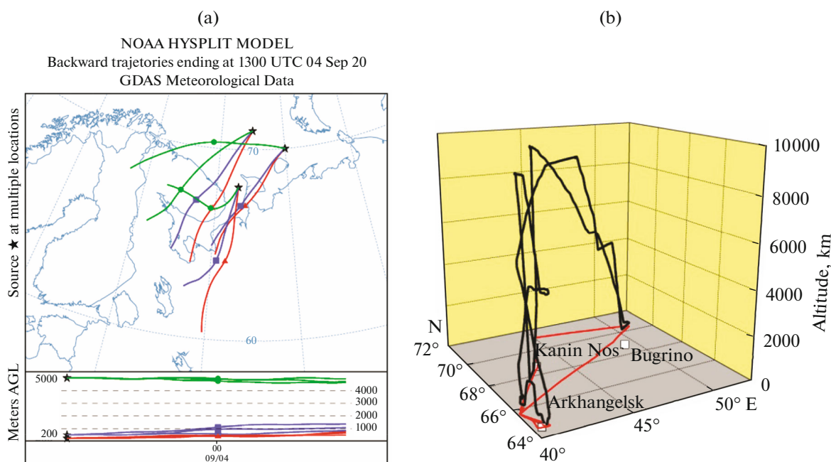
Fig. 3. (a) Back trajectories of air masses for the areas of measurement of vertical profiles of methane concentration (13:00–15:00 GMT, September 4, 2020); (b) pattern of the flight to the Barents Sea area.
