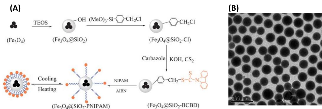
Figure 7. (A) Synthesis of core-shell RMPH hybrids by surface-initiated RAFT polymerization. In a first step, the \text{Fe}_3\text{O}_4 @ \text{SiO}_2 were functionalized with a RAFT agent via a silanization approach, (B) TEM images of the resulting \text{Fe}_3\text{O}_4 @ \text{SiO}_2 -PNIPAM NPs (reproduced from reference 91 with permission from the Royal Society of Chemistry)
