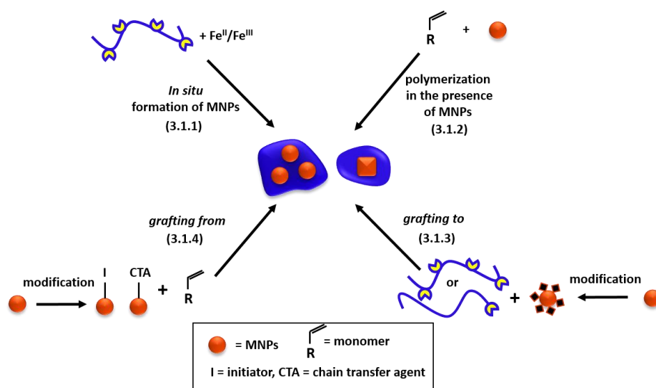
Figure 3. Summary of the different approaches used to prepare core-shell stimuli-RMPH.
