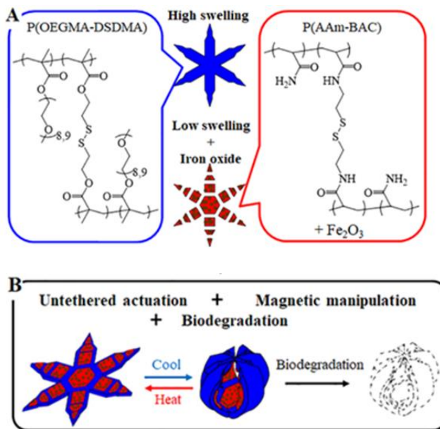
Figure 17. Schematic representation of the molecular composition, structure, and operation of the magneto-thermo-responsive grippers. (A) The grippers are composed of a bilayer of two hydrogels: a reversible high-swelling P(OEGMA-DSDMA) gel, and a low-swelling P(AAm-co-BAC) gel containing IONPs. (B) Illustration of the multifunctional nature of the soft grippers, including thermo-responsive actuation, magnetic manipulation, and biodegradation (adapted with permission from ACS Applied Material Interfaces, 2019, 11(1), 151-159, ©2018, American Chemical Society. 171 )
