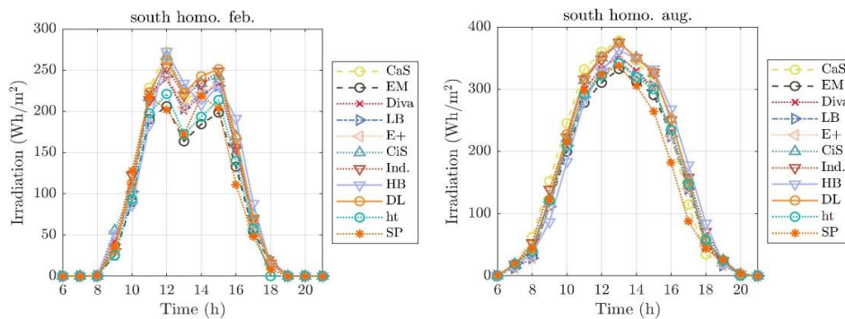
Figure 4: Irradiation on the southern face of the homogeneous district (left) February, (right) August
