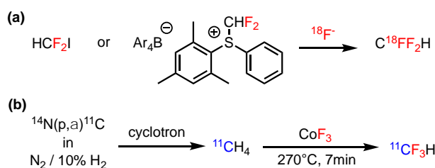
Scheme 15. Preparation of [ ^{18}\text{F} ] and [ ^{11}\text{C} ]fluoroform.
