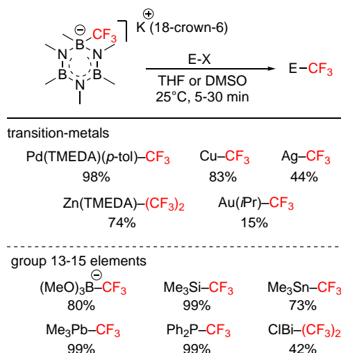
Scheme 12. Reactions of borazine-CF 3 reagent with inorganic electrophiles.
