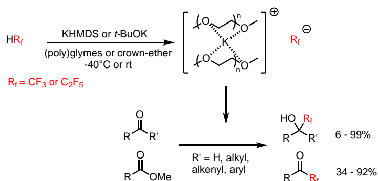
Scheme 4. Glymes and crown ethers to generate naked CF_3^- anion.
