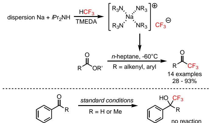
Scheme 6. \text{NaCF}_3 species in trifluoromethylation of aromatic esters.
