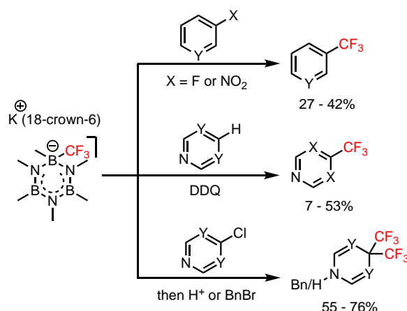
Scheme 14. Reactions of borazine- \text{CF}_3 reagent with (hetero)aryl substrates.
