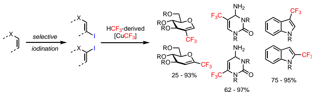
Scheme 7. Trifluoromethylation of alkenyl iodides from biomolecules.
