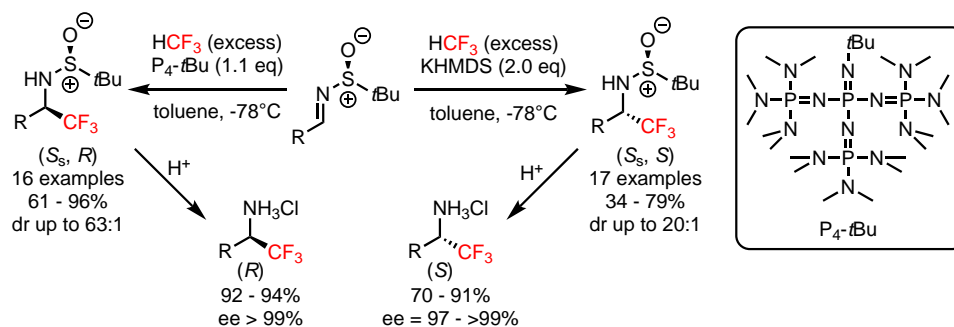
Scheme 1. Stereodivergent trifluoromethylation of N -sulfinylimines.
