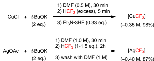
Scheme 8. Preparation of [\text{CuCF}_3] and [\text{AgCF}_3] reagents from fluoroform.
