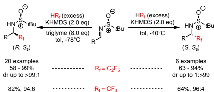
Scheme 5. KHMDS/triglyme cryptate as an alternative to P_4 - t Bu.
