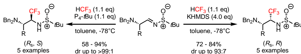
Scheme 2. Stereodivergent diastereoselective synthesis of enantioenriched trifluoromethylated ethylenediamines.
