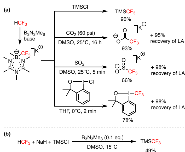
Scheme 11. Synthesis of \text{Me}_3\text{SiCF}_3 , \text{KSO}_2\text{CF}_3 , and Togni reagent from \text{HCF}_3 .
