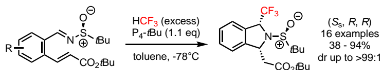
Scheme 3. Diastereoselective synthesis of enantioenriched isoindolines.
