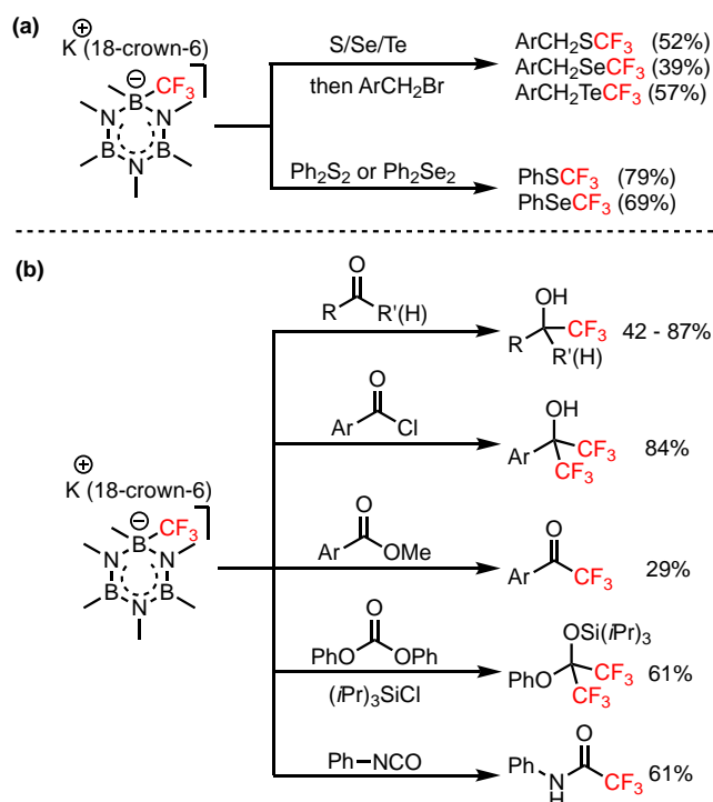
Scheme 13. Reactions of borazine-CF 3 reagent with (a) organic and inorganic chalcogens (b) carbonyl compounds.
