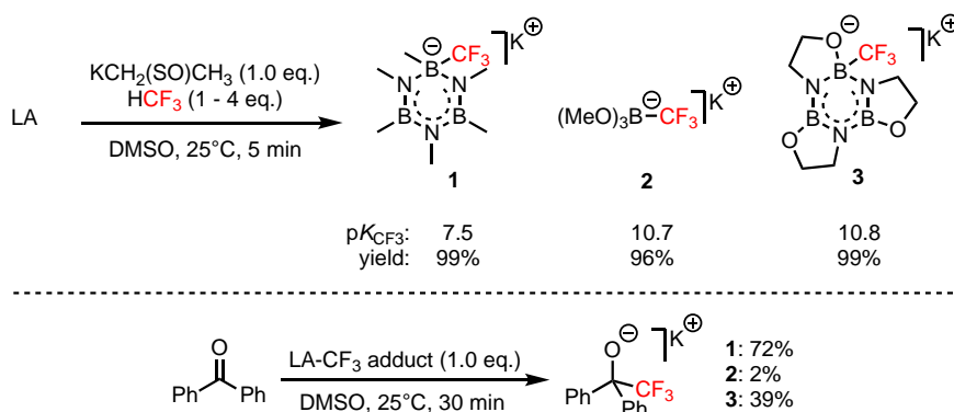
Scheme 10. Trifluoromethylation reagents from boron-based Lewis acids and fluoroform.
