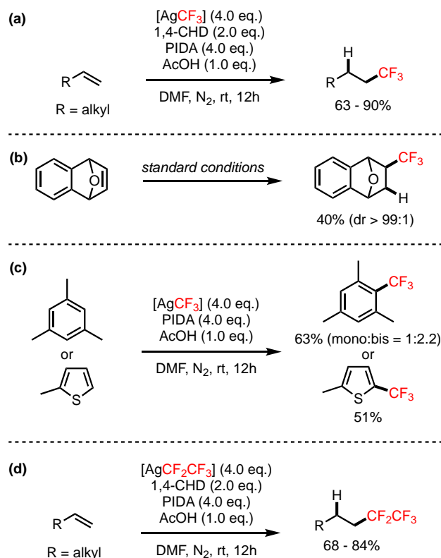
Scheme 9. Applications of [\text{AgCF}_3] and [\text{AgCF}_2\text{CF}_3] reagents.
