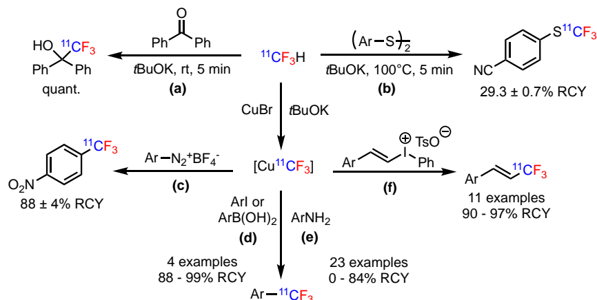
Scheme 16. Applications of [ ^{11}\text{C} ]fluoroform.
