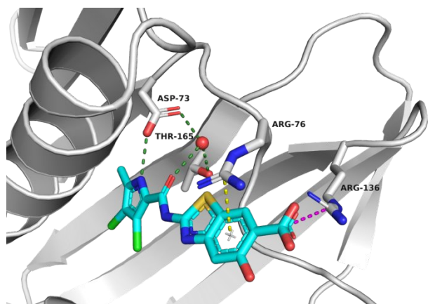
Figure 3: Cocystal structure of compound A (in cyan sticks) in the ATP-binding site of E. coli DNA gyrase B (in grey cartoon; PDB ID 7P2N). The ligand and the amino acid residues that interact with it are shown as stick models, and coloured according to atom type (blue, N; red, O; light green, Cl; brown, S). The water molecule is presented as a red sphere, hydrogen bonds are indicated by green dotted lines, the salt bridge is indicated by the magenta dotted line and the cation- \pi interaction by a yellow dotted line.
