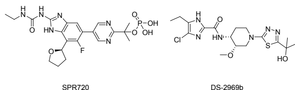
Figure 1: Structures of fobrepodacin (SPR720) and DS-2969b.
