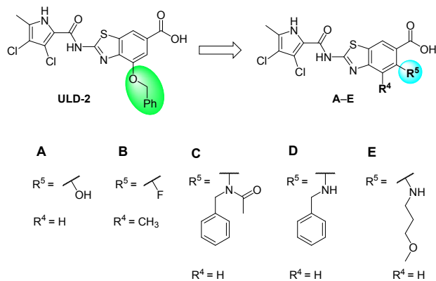
Figure 2: New series of compounds A-E with substitution at C5 position of the benzothiazole scaffold.
