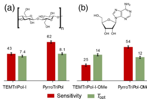
Fig. 7 Experimental sensitivity (red), optimal recycling delay for sensitivity, T_{\text{opt}} , as defined in ref. 34 and ESI† (green) measured for (a) cellulose microcrystalline powder impregnated with 10 mM TEMTriPol-I and PyrroTriPol in d_8 -glycerol/ D_2O/H_2O (60 : 30 : 10 v/v) and for adenosine microcrystalline powder impregnated with (b) 16 mM TEMTriPol-I-OMe and PyrroTriPol-OMe. All the data were recorded at 9.4 T, 8 kHz MAS and 110 K. Chemical structures of (a) cellulose and (b) adenosine are shown above the data plots.
