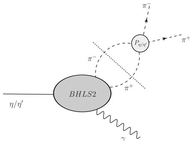
Figure 3: Diagram sketching the sharing between BHLS_2 and the Final State Interaction process in the \eta/\eta' decays to \pi^+\pi^-\gamma . In the global fit context, T_X(s) , represented by the lower blob, takes care of the non-perturbative effects. The drawing somewhat anticipates about the P_X(s) universality.
