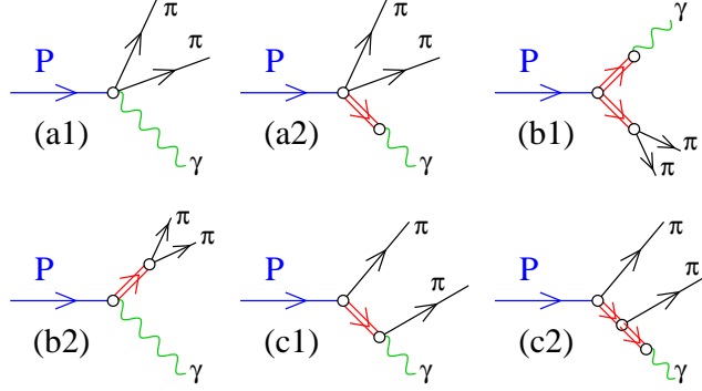
Figure 1: The classes of tree diagrams. P stands for either of \eta and \eta' ; in diagrams a and b , the double lines stand for the neutral vector mesons (subject to mixing), in diagrams c , the intermediate vector meson is \rho^\pm whereas the external one is neutral. The pions are charged. The vanishing of the AVP couplings (see text) implies that diagrams (b2) and (c1) do not contribute to the decay amplitudes.
