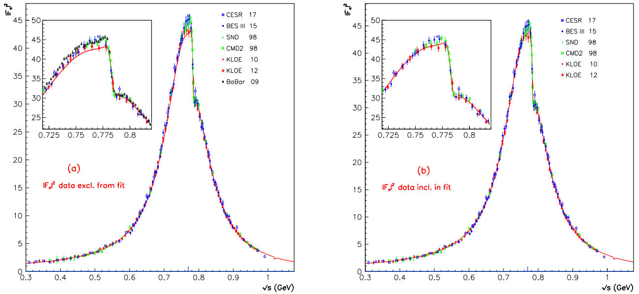
Figure 8: The curve displayed in the left-side panel (a) is the pion form factor predicted by fitting the data sample set \{\mathcal{X}_\tau + \eta/\eta'\} and, superimposed, the unfitted pion form factor spectra (including those from BaBar). The right-hand side panel (b) shows the pion form factor derived from fitting the full \{\mathcal{H}_R + \eta/\eta'\} data sample set which includes the KLOE and NSK pion form factors (but not the BaBar spectrum). See the text for comments.
