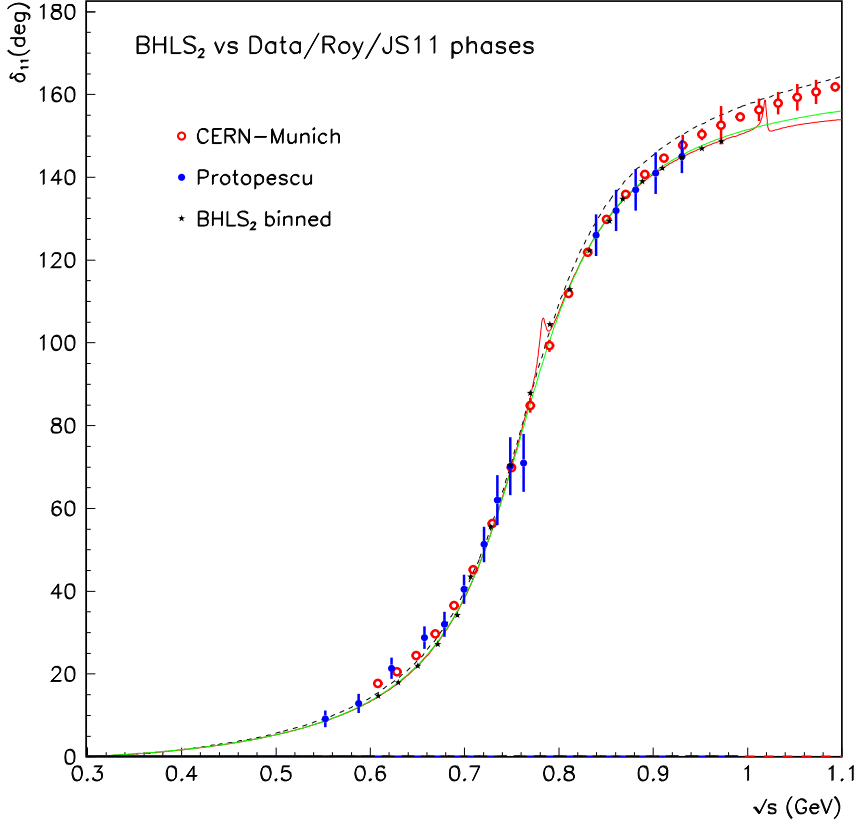
Figure 2: The \delta_{11} phase-shift plotted as function of \sqrt{s} . Beside the data points of [69, 70], the dashed black curve is the solution to the Roy Equations [71], the green full line shows the phase reconstructed in [72] and red full line the BHLS 2 phase-shift exhibiting the \omega and \phi signals. The black stars show the smeared BHLS 2 spectrum (e.g. the red curve).
