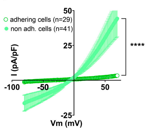
Figure 3. Expression of E or 3a protein is accompanied by outwardly rectifying currents in non-adhering CHO cells only. Left , average current densities ( \pm sem) recorded during the ramp protocol in adhering (empty circles) or non-adhering (filled circles) CHO cells expressing either eGFP ((A), pIRES), SARS-CoV-2 E and eGFP proteins ((B), pIRES-E) or SARS-CoV-2 3a and eGFP proteins ((C), pIRES-3a). Right , plot of the individual adhering cells (darker color) or non-adhering cells (lighter color). ****: p < 0.0001 , compared to adhering cells, two-way ANOVA on Ranks.
