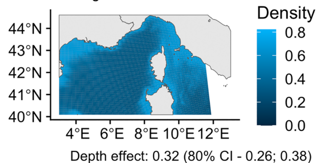
Figure 2 Estimated density surfaces of bottlenose dolphins ( Tursiops truncatus ) for the three models. Lighter colour indicates more individuals per area unit. Both spatial integrated model (SIM) and distance sampling model (DS) predicted higher density in coastal seas, while spatial capture–recapture model (SCR) predicted homogeneous density across the study area. Note that density scales are different between the maps, indicating a higher overall population size for the DS model than for SIM and SCR model.
