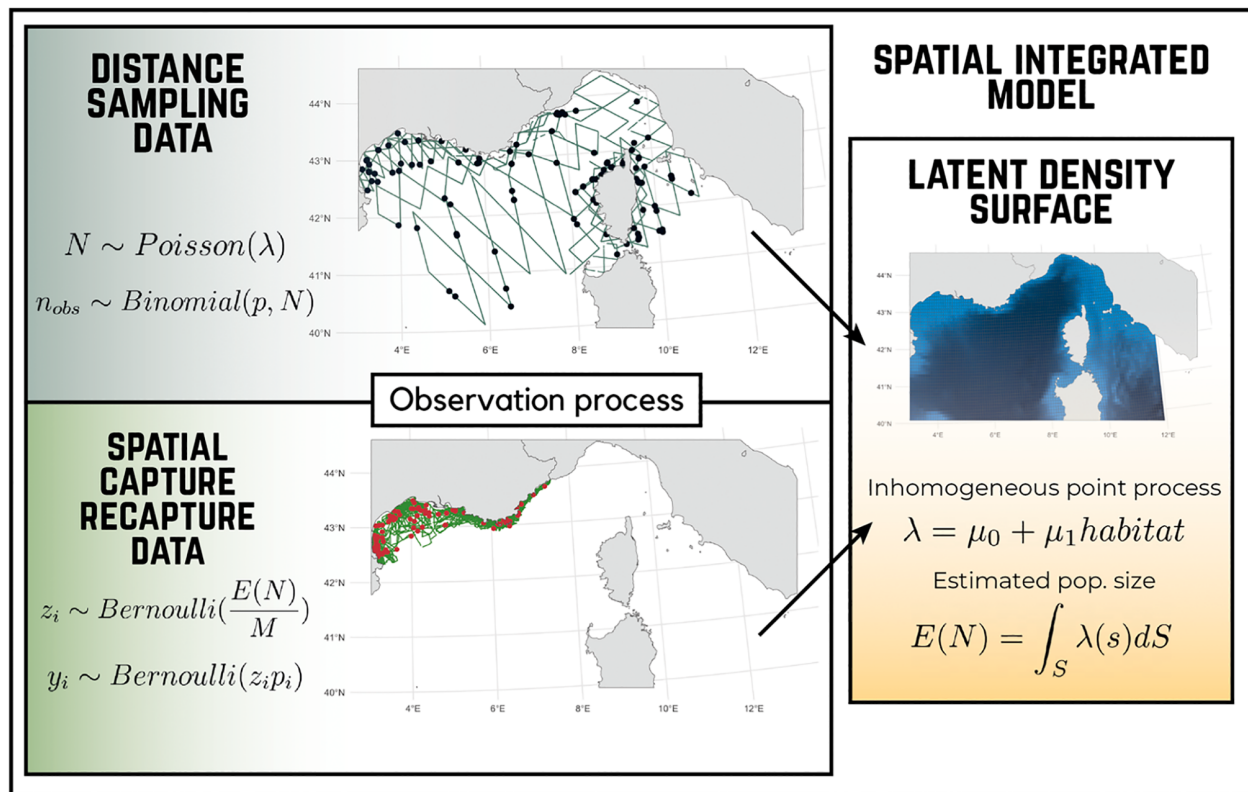
Figure 1 Graphical description of the spatial integrated model (SIM) that combines spatial capture–recapture (SCR) and distance sampling (DS) of bottlenose dolphins. The SIM is a hierarchical model with three processes: i) latent population size E(N) and density \lambda informed by an inhomogeneous point process, ii) DS observation process that links the line transect dataset to the latent density surface and iii) SCR observation process that links the detection histories to the latent density. The observation process is stochastic according to detection probability. For DS model, the observed group size n_{obs} is a binomial draw in the latent abundance N at the sample grid cell. For SCR model, observing an individual
