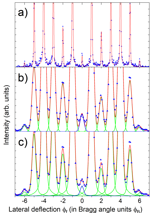
FIG. 10. Diffracted intensities recorded with He on LiF [110] at (a) 300 eV, \theta_i=1.35^\circ and (b,c) 5000 eV and \theta_i=0.33^\circ . Both correspond to E_\perp \sim 165 meV and were recorded with an angular resolution 0.007^\circ ( 0.016^\circ FWHM). The red lines correspond to a fit through the data using a common line shape for all peaks. (b) is fitted by a pure Gaussian while (a) and (c) correspond to the profile E^*(\phi) in Table II. The contribution of the specular peak (blue line) depends on the line shape.
