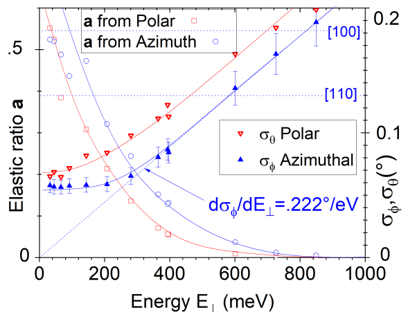
FIG. 7. Evolution of the azimuthal \sigma_\phi ( \blacktriangle ) and polar \sigma_\theta ( \nabla ) widths during a \theta -scan at E=500 eV along a [Rnd] direction where only the specular peak is present. The coefficient a in eq. (1) represents the elastic ratio extracted from a fit of the azimuthal ( \circ ) or of the polar profile ( \square ). The lines are to guide the eyes.
