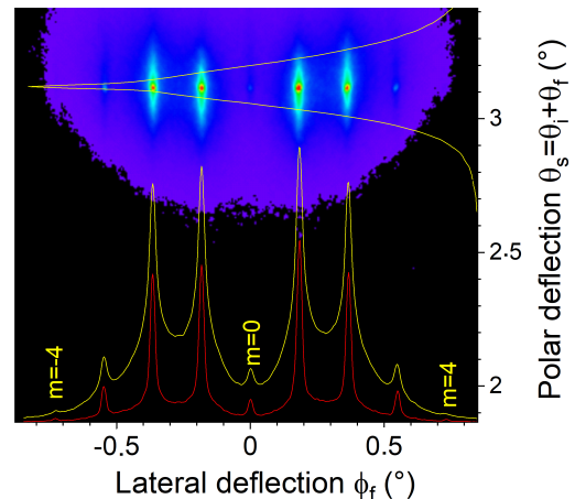
FIG. 2. The raw plot in Fig. 1 is polar transformed following Ref. [5]. The yellow lines are the overall polar and azimuthal profiles corresponding to intensity projections (full integration) while the red one is the intensity ( \times 20 ) of a 0.015^\circ band at the specular angle ( \theta_f = \theta_i ).
