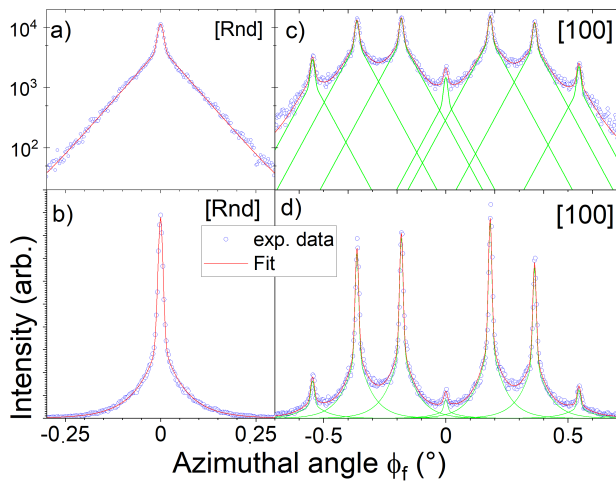
FIG. 4. The scattering pattern of 500 eV He atoms impinging at \theta_i=1.54^\circ ( E_\perp=365 meV) on LiF at T=180 K. Left panels (a,b) are for a random direction while the right ones (c,d) are for a [100] direction. Top panels (a,c) are in log scale. Both directions are well-fitted with a unique lineshape, the a value indicates an inelastic ratio of 83% while the exponential decay range \phi_0 is here 0.06^\circ .
