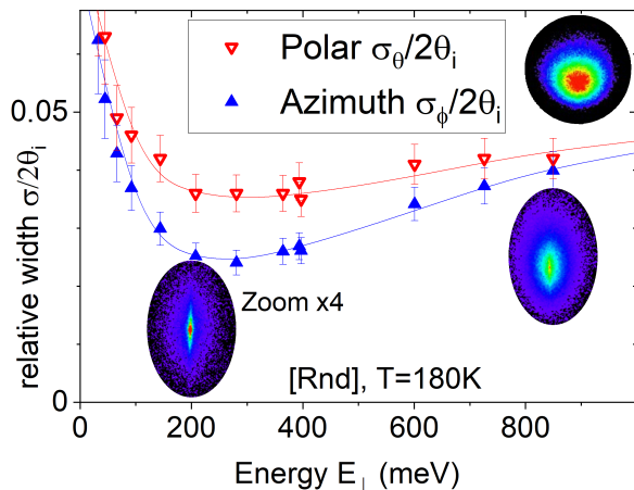
FIG. 8. The same polar and azimuthal widths as in Fig. 7 are plotted as a dimensionless relative widths \sigma_\phi/2\theta_i ( \blacktriangle ) and \sigma_\theta/2\theta_i ( \blacktriangledown ) used in Ref. [7, 38]. The lines are to guide the eyes. Inserts are 2D( \phi, \theta ) profiles at E_\perp=200 and 850 meV, the one in the upper right corner was recorded separately at 3 keV and 3.5^\circ ( E_\perp \simeq 10 eV) and is compressed 9 times.
