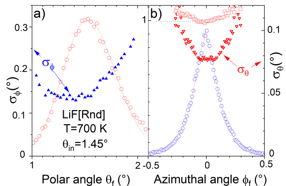
FIG. 12. For 500 eV helium scattered along a [Rnd] direction at \theta_i=1.45^\circ incidence ( E_\perp = 320 meV and E\theta^3=8.1 meV), the polar \circ (a) and azimuthal \circ (b) profiles are reported showing no clear elastic component. The standard deviation of the azimuthal \blacktriangle and polar \blacktriangledown distributions show a diffuse minimum and a possible quadratic dependence. The \square symbols represent \bar{\theta}_f/\theta_i and show the weak variation of the mean polar scattering angle.
