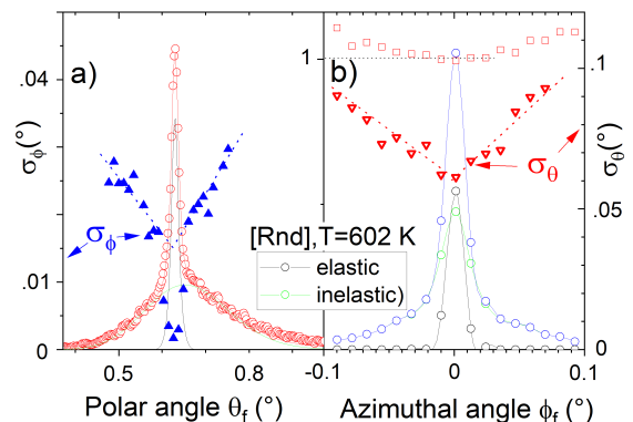
FIG. 11. For 500 eV helium scattered along a [Rnd] direction at \theta_i=0.628^\circ incidence ( E_\perp = 60 meV and E\theta^3=0.66 meV), the polar \circ (a) and azimuthal \circ (b) profiles are decomposed into elastic \circ and inelastic \triangle components. The standard deviation of the azimuthal \blacktriangle and polar \blacktriangledown distributions show a linear increase away from elastic conditions, dotted lines are to guide the eyes. The \square symbol represents \bar{\theta}_f/\theta_i and shows the weak variation of the mean polar scattering angle.
