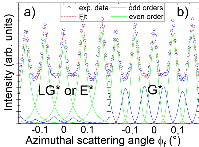
FIG. 9. The central part of the diffracted intensities along LiF [110] at 5 keV and 0.75^\circ ( E_\perp=865 meV) is fitted by two line profiles of Table II. (a) L.G^* ( E^* gives equivalent results) (b) G^* . The odd diffraction orders in blue are expected to be weak (see text) and this is better reproduced by the fit in (a). The elastic weight is estimated at around 5% from the polar profile and is hardly visible here.
