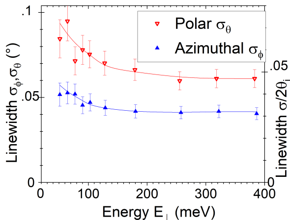
FIG. 6. The Polar ( \sigma_\theta \nabla ) and azimuthal ( \sigma_\phi \blacktriangle ) widths of the overall inelastic profile recorded along a [Rnd] direction during an E -scan at a fixed incidence angle \theta_i=0.66^\circ are reported as a function of the perpendicular energy E_\perp with lines to guide the eyes. The scale on the right-hand side shows the dimensionless unit \sigma/2\theta_i used in Ref. [7, 38, 41].
