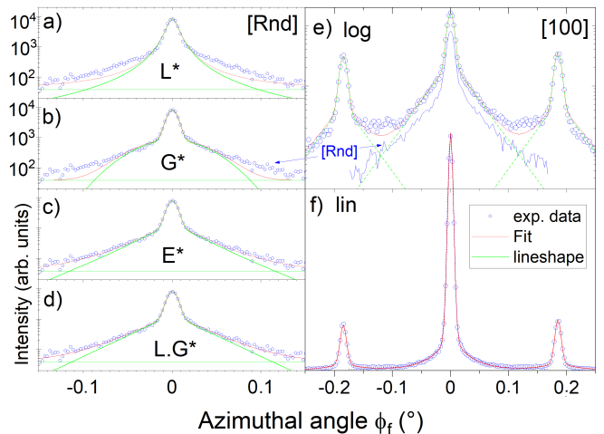
FIG. 3. The scattering patterns of 500 eV He atoms impinging at \theta_i=0.66^\circ ( E_{\perp}=66 \text{ meV} , E\theta^3=0.76 \text{ meV} ) on LiF at T=180\text{K} . The left panels (a)-(d) are for a random direction [Rnd] compared with a Lorentzian, Gaussian, Exponential, and bounded Lorentzian, respectively. The right ones are for a [100] direction in linear (f) and log scale (e). The blue line in (e) is the raw profile in (a)-(d) while the green lines in (e) and (d) are the convolution of a pure exponential decay with a range \phi_0 = 0.031^\circ by the beam profile with \sigma_b=0.006^\circ . f(\phi)^* = (0.52 \delta(\phi) + 0.48 A e^{-|\phi/\phi_0|}) * e^{-\phi^2/2\sigma_b^2} .
