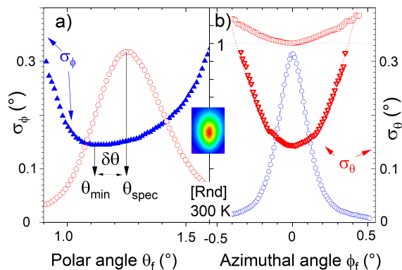
FIG. 13. Same as Fig. 11 and 12 with 4 keV He projectiles at 1.25^\circ ( E\theta^2=1.9 eV, E\theta^3=41 meV). No elastic component is visible in the polar \circ (a) and azimuthal \circ (b) profiles. The standard deviation \sigma_{\phi\blacktriangle} of the azimuthal distribution associated with a polar angle \theta_f shows a minimum located at \theta_{min} well below the specular scattering angle \theta_{spec} . The polar width \sigma_\theta \blacktriangledown has a quadratic behavior ( \sigma_\phi \sim 0.14 + 1.4\phi_f^2 ). The mean scattering angle \bar{\theta}_f/\theta_i ( \square ) varies weakly with \phi as in Figs. 11-12.
