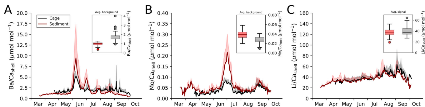
Fig. 1. Averaged Ba/Ca_{shell} (A), Mo/Ca_{shell} (B), and Li/Ca_{shell} (C) profiles ( +1\sigma ) obtained from three Pecten maximus specimens grown inside a cage (black) and on the sediment surface (red) during 2021. Box plots indicate differences in the background signals between cage and sediment shells of average Ba/Ca_{shell} and Mo/Ca_{shell} profiles and the average signal of Li/Ca_{shell} ratios.
