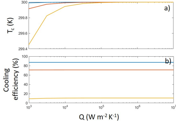
FIG. 6. (a) Carrier temperature T_c and (b) cooling efficiency \eta_{cooling} versus the electron-phonon scattering parameter Q for incident laser power of (blue) 1 \text{ mW.cm}^{-2} , (red) 10 \text{ mW.cm}^{-2} and (yellow) 100 \text{ mW.cm}^{-2} .
