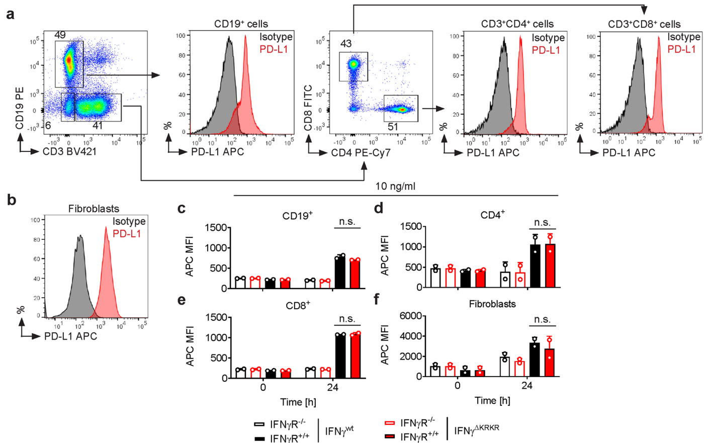
Extended Data Fig. 7 | Similar upregulation of PD-L1 by IFN \gamma and IFN \gamma^{\Delta KRKR} . Splenocytes or fibroblasts were cultured in the presence of 10 ng/ml IFN \gamma or IFN \gamma^{\Delta KRKR} . Cells were analyzed 24 h after cytokine exposure for PD-L1 expression. a , Gating strategy for splenocytes, and b , Example staining of fibroblasts cultured with IFN \gamma . c , CD19 + ; d , CD4 + ; e , CD8 + ; and f , fibroblasts are shown.
