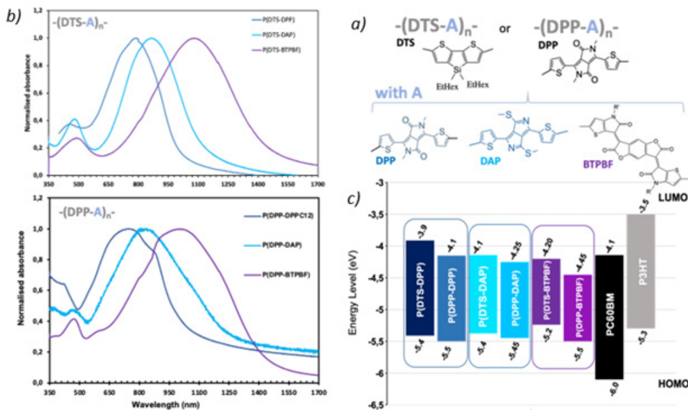
Figure 1: a) chemical structures of compared D-A and A-A copolymer; b) UV-visible-NIR absorption spectra of thin films; c) electronic levels determined from cyclic voltametry.
