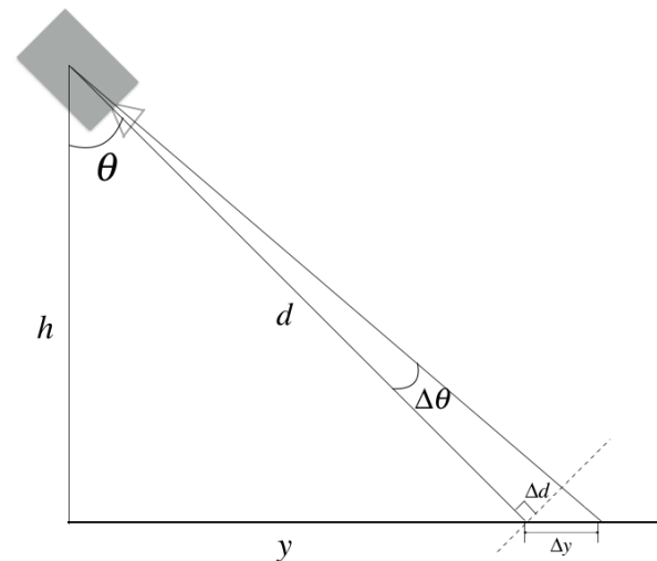
Figure 4: System geometry
