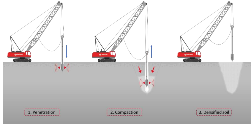
Fig. 1. Vibro compaction process.
