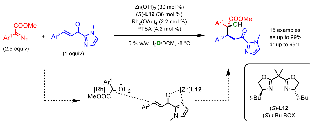
Scheme 8: Synergistic Rh/Zn multicomponent transformation
