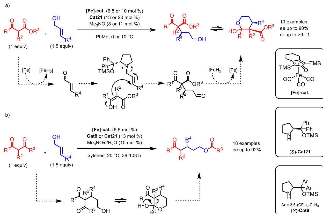
Scheme 37: Enantioselective multicyclic borrowing hydrogen and application in a cascade Claisen fragmentation
