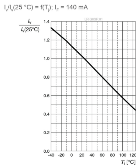
Figure 7. Relative luminous intensity as a function of the junction temperature [37].
