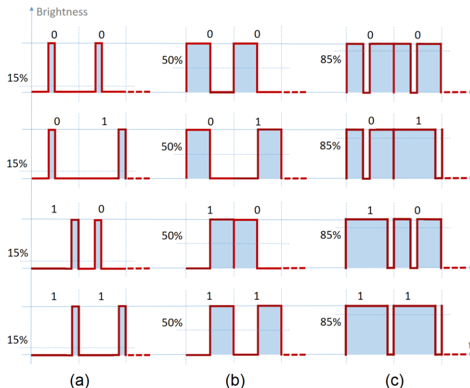
Figure 1. The modified VPPM coding scheme implemented in [34]: (a) Average illumination less than 50%; (b) Average illumination equal to 50%, the same as Manchester coding; (c) Average illumination greater than 50%.
