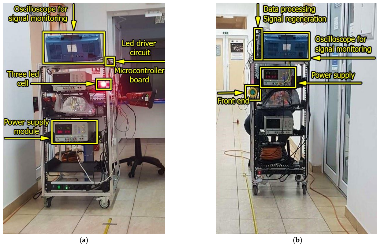
Figure 6. Hardware implementation of the VLC prototype used for the range extension experiments: (a) VLC emitter; (b) VLC receiver.
