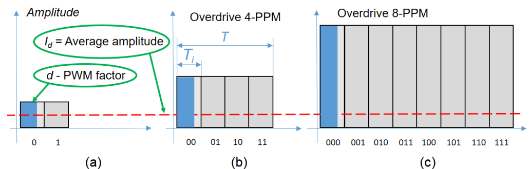
Figure 3. Theoretical analysis for overdriving an LED with a reduced duty factor, using VPPM: (a) Manchester code; (b) 4-PPM; (c) 8-PPM.
