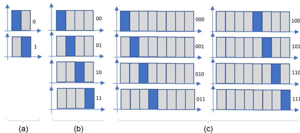
Figure 2. n -PPM examples: (a) n = 2 , binary PPM (Manchester code); (b) n = 4 , 4-ary PPM; (c) n = 8 , 8-ary PPM.
