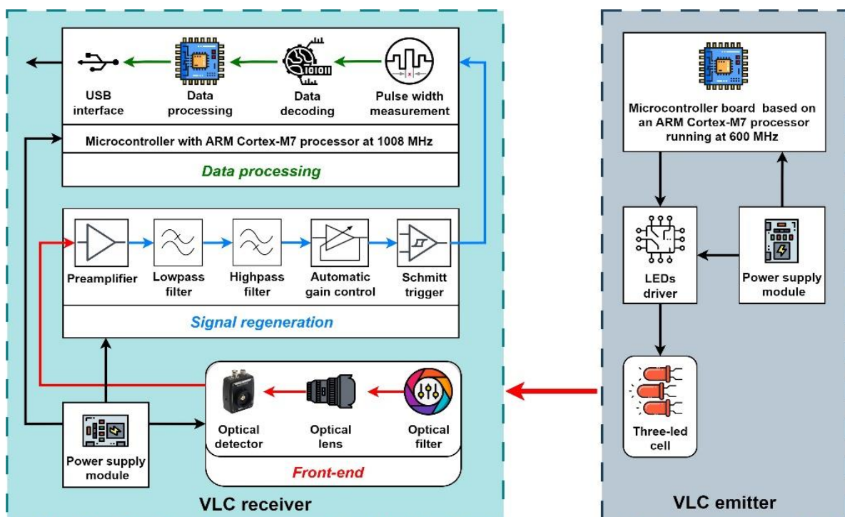
Figure 5. Schematic representation of the VLC prototype system used for the range extension experiments.
