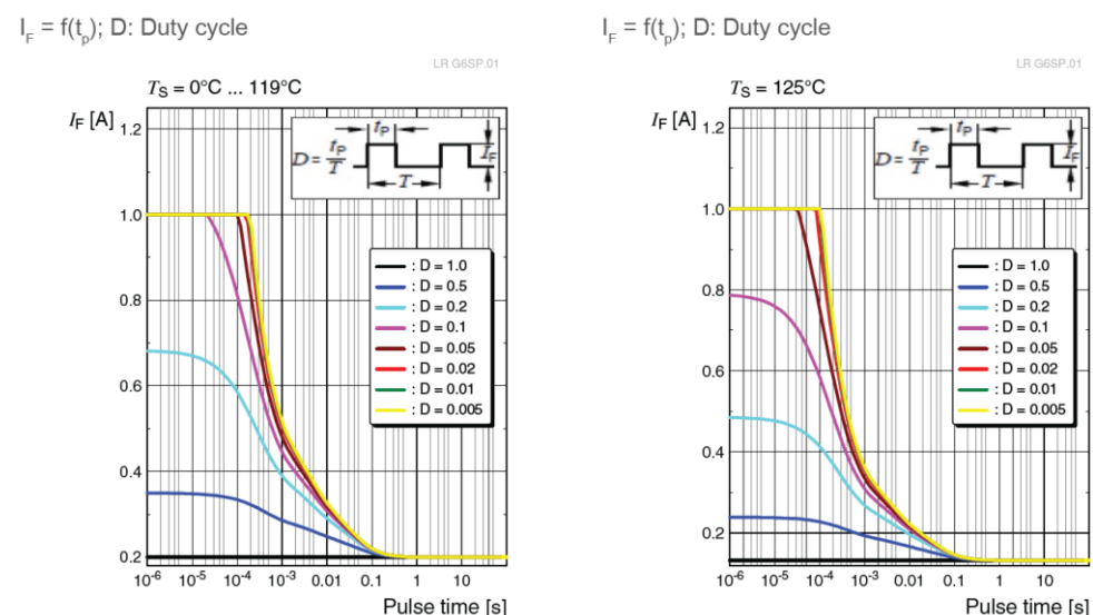
Figure 4. Pulse handling capability of an LR G6SP.01 LED up to 119 °C and for 125 °C [37].
