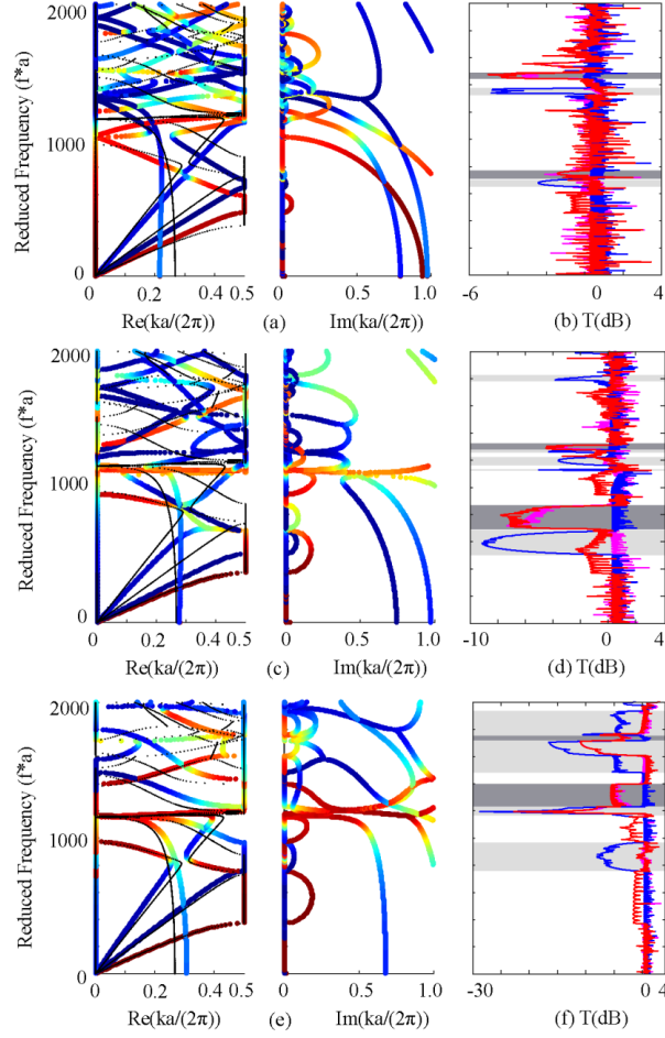
Figure 6: Influence of the normalized radius r/a and elastic material parameters on the complex band structure and the frequency response for the P/E system (elastic inclusion in a poroelastic matrix). Panels (a,b) present results for r/a = 0.2 . Panels (c,d) and (e,f) present results for epoxy and aluminum, respectively. Black dots are the real parts of the complex band structure for the concrete inclusion [Fig. 2(a)]. The color scale indicates wave polarization varying from blue (0) to red (1). The red, blue, and pink solid lines are for the responses to incident signals (1,0,0), (0,1,0), and (0,0,1), respectively. The light gray regions represent the band gaps for the SV wave in the complex band structure, whereas the gray regions show the band gaps for the two longitudinal waves.
