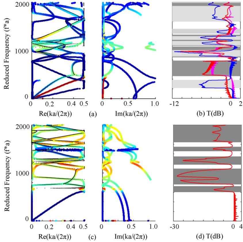
Figure 17: Influence of the pore fluid viscosity on complex band structure and transmission spectrum for 2D fluid and poroelastic metamaterials with the sealed-pore interface. Panels (a) and (c) present the variation of the real and imaginary wave numbers with the reduced frequency for P/F and F/P systems, respectively. Black dots present the real part of the complex band structure for an inviscid pore fluid. Panels (b) and (d) represent the frequency response functions for P/F and F/P systems, respectively. The line types and the light and gray regions are similar to the inviscid fluid case.
