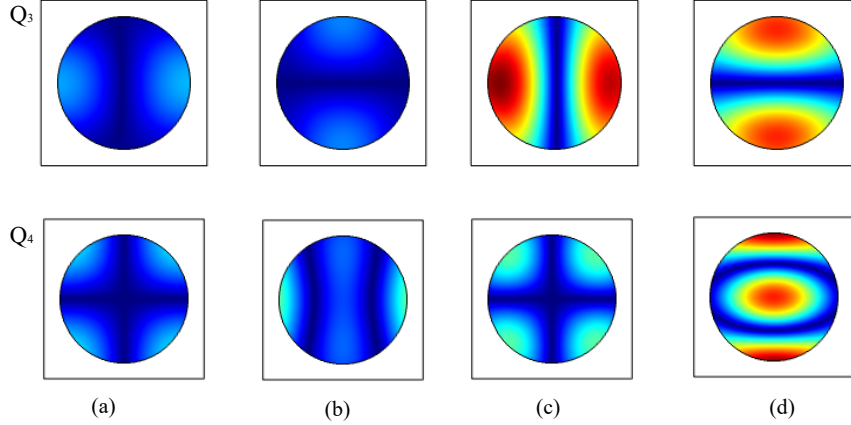
Figure 10: Modal distributions at marked points Q_3 and Q_4 in Figs. 9(c,d). Panels (a), (b), (c), and (d) show normalized displacements |u_x|/u_{\max} , |u_z|/u_{\max} , |U_x|/u_{\max} , |U_z|/u_{\max} , respectively. u_{\max} = \max(|u_x|, |u_z|, |U_x|, |U_z|) at every marked point. The color scale is the same as in Fig. 3.
