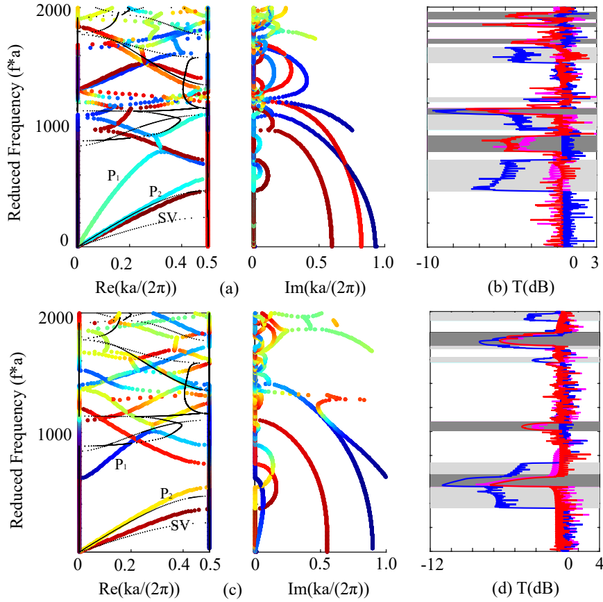
Figure 14: Influence of the normalized radius r/a on the complex band structure and the frequency response for the P/F system (fluid inclusion in a poroelastic matrix) with the open-pore interface. Panels (a,b) and panels (c,d) show the results for r/a = 0.2 and 0.3 , respectively. The color scale indicates the ratio of the kinetic energy of the pore fluid to the total kinetic energy in the matrix, from 0 (blue) to 1 (red). The black dots show the real part for r/a = 0.4 . The red, blue, and pink solid lines are for the responses to excitation signals (1,0,0) , (0,1,0) , and (0,0,1) , respectively. Light gray regions represent band gaps for SV waves, whereas gray regions represent band gaps for two longitudinal waves.
