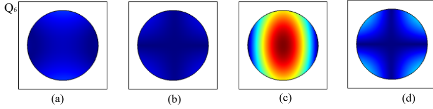
Figure 13: Modal distribution at the marked point ( Q_6 ) in Fig. 12(a). Panels (a), (b), (c), and (d) show the normalized displacements |u_x|/u_{\max} , |u_z|/u_{\max} , |U_x|/u_{\max} , |U_z|/u_{\max} , respectively. u_{\max} = \max(|u_x|, |u_z|, |U_x|, |U_z|) at marked point. The color scale is the same as in Fig. 3.
