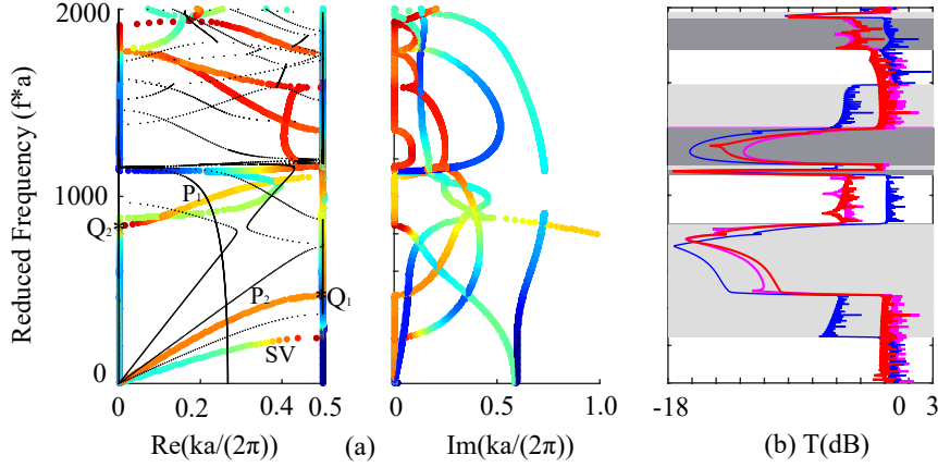
Figure 8: Complex band structure and transmission for the P/F system (fluid inclusion in a poroelastic matrix) with the open-pore interface. The left and right parts in panel (a) stand for the relation of the reduced frequency with the real and imaginary parts of the wave number. The color scale indicates the ratio of the kinetic energy of the pore fluid to the total kinetic energy in the matrix, ranging from 0 (blue) to 1 (red). The black dots are the real part of the complex band structure for the P/E system. The calculated transmission spectrum is plotted in panel (b). The red, blue, and pink solid lines are for the responses to incident signals (1,0,0), (0,1,0) and (0,0,1), respectively. Light gray regions represent band gaps for SV waves, whereas gray regions represent band gaps for P waves.
