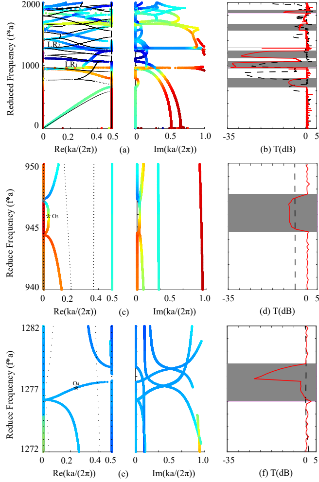
Figure 9: Complex band structure and transmission for the F/P system (poroelastic inclusion in a fluid matrix) with the open-pore interface. The left and right parts in panel (a) stand for the relation of the reduced frequency with the real and imaginary parts of the wave number. The color scale indicates the ratio of the kinetic energy of the pore fluid to the total kinetic energy of the inclusion, from 0 (blue) to 1 (red). Black dots present the real part of the complex band structure of the associated 2D fluid/solid system with the solid skeleton parameters of the poroelastic inclusion used for the solid. The calculated transmission spectrum is plotted in panel (b). Red solid lines present the received signal \log_{10} |p| under the unit excitation ( p_0 = 1 ). Black dashed lines present the transmission of the fluid/solid system. Gray regions indicate band gaps for longitudinal waves. Panels (c-f) are zoomed complex band structures and transmission in the reduced frequency regions 940 m/s - 950 m/s and 1272 m/s - 1282 m/s.
