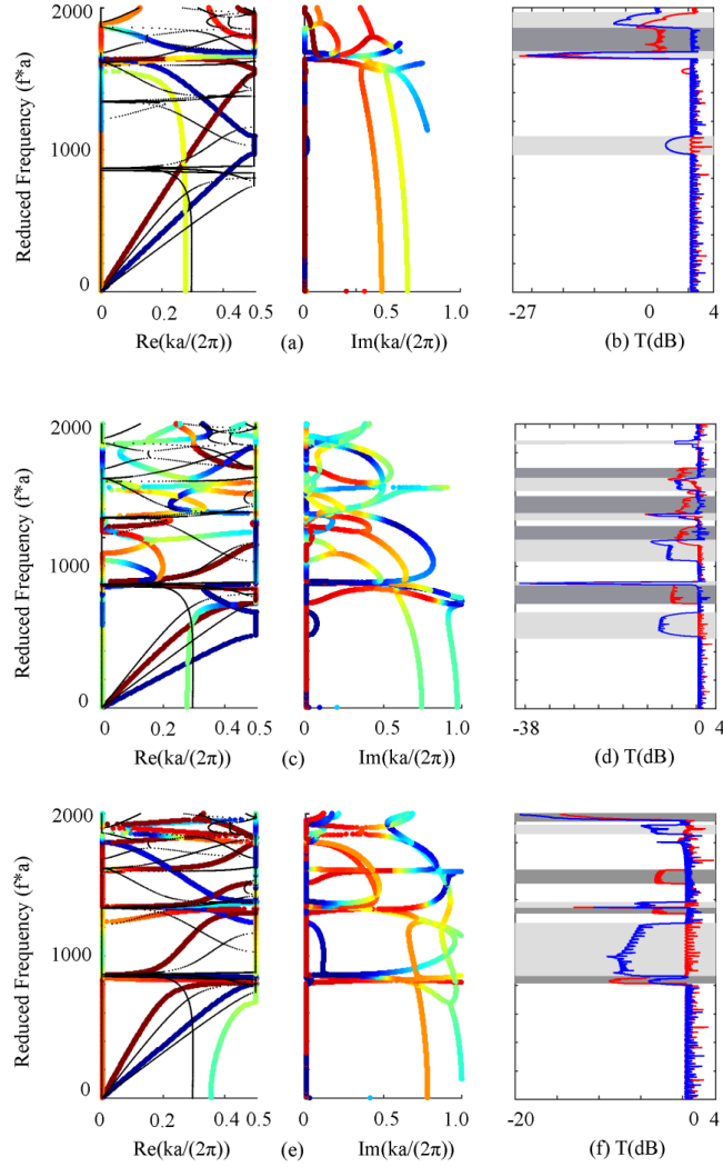
Figure 7: Influence of normalized radius r/a and elastic material parameters on the complex band structure and the frequency response for the E/P system (poroelastic inclusion in an elastic matrix). Panels (a,b) present results for r/a = 0.2 . Panels (c,d) and panels (e,f) present results for epoxy and aluminum for r/a = 0.4 . The black points are the real parts of the complex band structure for the concrete matrix [Fig. 4(a)]. The color scale indicates wave polarization varying from blue (0) to red (1). Light gray regions represent band gaps for SV waves, whereas gray regions represent band gaps for P waves.
