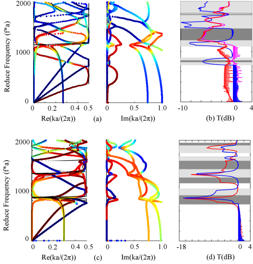
Figure 16: Influence of the pore fluid viscosity on complex band structure and transmission spectrum for the poroelastic/elastic interface. Panels (a) and (c) present the variation of the real and imaginary wave numbers with the reduced frequency for P/E and E/P systems, respectively. Black dots present the real part of the complex band structure for an inviscid pore fluid. The color scales are the same as in Fig. 2(a) and Fig. 4(a), respectively. Panels (b) and (d) represent the frequency response functions for P/E and E/P systems, respectively. The line types and the light gray and gray regions are similar to the inviscid fluid case.
