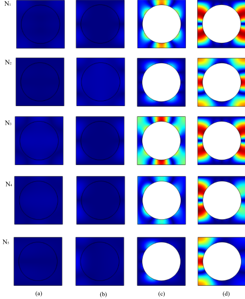
Figure 3: Modal distributions at marked points ( N_1, N_2, N_3, N_4, N_5 ) in Fig. 2(a). Panels (a), (b), (c), and (d) show the normalized displacements |u_x|/u_{\max} , |u_z|/u_{\max} , |U_x|/u_{\max} , |U_z|/u_{\max} , respectively. u_{\max} = \max(|u_x|, |u_z|, |U_x|, |U_z|) at every marked point. The color scale represents the normalized displacement amplitude ranging from 0 (blue) to 1 (red).
