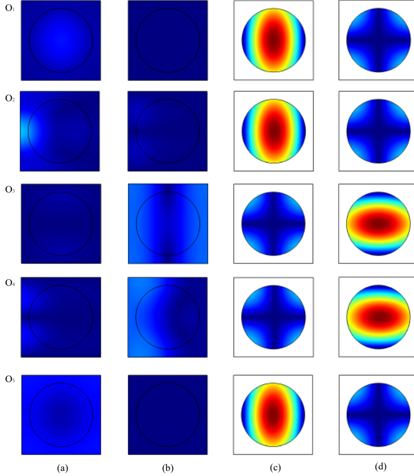
Figure 5: Modal distributions at marked points ( O_1, O_2, O_3, O_4, O_5 ) in Fig. 4(c). Panels (a), (b), (c), and (d) show the normalized displacements |u_x|/u_{\max} , |u_z|/u_{\max} , |U_x|/u_{\max} , |U_z|/u_{\max} , respectively. u_{\max} = \max(|u_x|, |u_z|, |U_x|, |U_z|) at every marked point. The color scale is the same as in Fig. 3.
