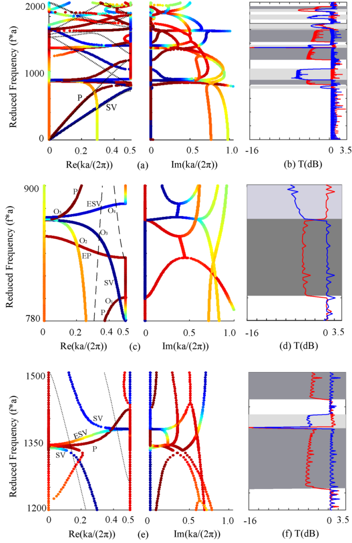
Figure 4: Complex band structures and transmission for the E/P system (poroelastic inclusion in an elastic matrix). Panel (a) shows the complex band structure or the dependence of the reduced frequency with the real and imaginary parts of the wave number. Black dots represent the real band structure of a 2D solid/solid structure with constant geometric parameters. The color scale indicates the ratio of the kinetic energy in the x direction to the total kinetic energy in the matrix, ranging from 0 (blue) to 1 (red). Light gray regions represent band gaps for SV waves, whereas gray regions represent band gaps for P waves. Panels (c) and (e) are zoomed complex band structures, and panels (d) and (f) are zoomed frequency responses of panels (a) and (b), for the reduced frequency ranges 780 m/s - 900 m/s and 1200 m/s - 1500 m/s, respectively
