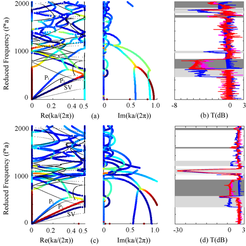
Figure 15: Influence of the normalized radius r/a on the complex band structure and the frequency response for the P/F system (fluid inclusion in a poroelastic matrix) with the sealed-pore interface. Panels (a,b) and panels (c,d) show the results for r/a = 0.2 and 0.3 , respectively. The color scale indicates the ratio of the kinetic energy of the pore fluid to the total kinetic energy in the matrix, from 0 (blue) to 1 (red). The black dots show the real part for r/a = 0.4 . The red, blue, and pink solid lines are for the responses to excitation signals (1,0,0) , (0,1,0) , and (0,0,1) , respectively. Light gray regions represent band gaps for SV waves, whereas gray regions represent band gaps for the two longitudinal waves.
