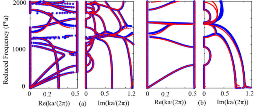
Figure B.18: Blue stars and red dots of panel (a) are the complex band structures for the P/P and the P/E systems; respectively. Blue stars and red dots of panel (b) are the complex band structures for the P/P and the fluid/solid systems; respectively.
