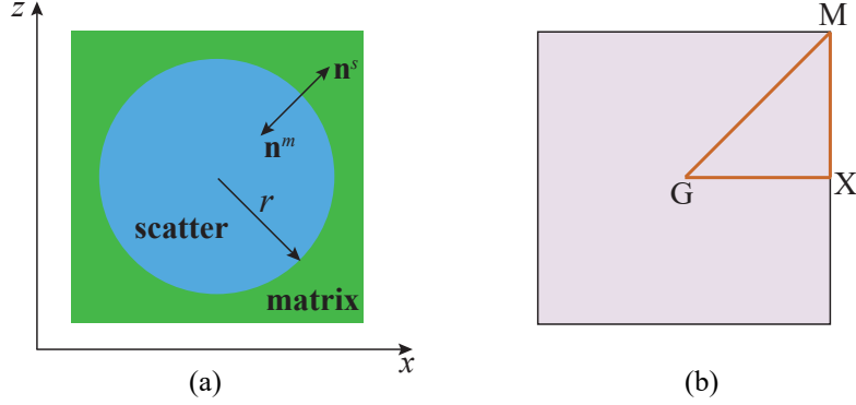
Figure 1: 2D square-lattice metamaterial of circular inclusions embedded in a matrix. (a) Schematic diagram of the unit cell. The metamaterial is assumed infinite along the y -axis and periodic in the (x,z) plane. (b) Sketch of the corresponding first Brillouin zone.
