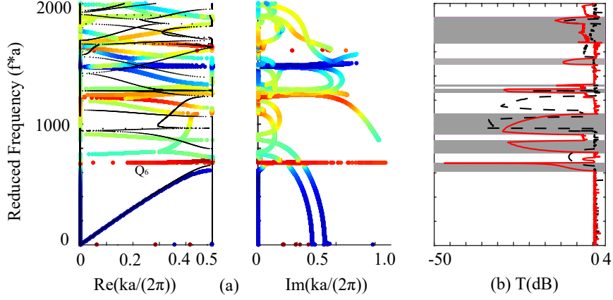
Figure 12: Complex band structure and transmission spectrum for the F/P system (poroelastic inclusion in a fluid matrix) with the sealed-pore interface. The left and right parts in panel (a) display the relation of the reduced frequency with the real and imaginary parts of the wave number. The color scale indicates the ratio of the kinetic energy of the pore fluid to the total kinetic energy of the inclusion, from 0 (blue) to 1 (red). The black dots present the real part of the complex band structure for the F/P system with the open-pore interface. The calculated transmission spectrum is plotted in panel (b). The red solid line is for the received signal \log_{10} |p| under a unit excitation. The black dashed line is for the transmission of the open-pore interface. Gray regions indicate band gaps for longitudinal waves.
