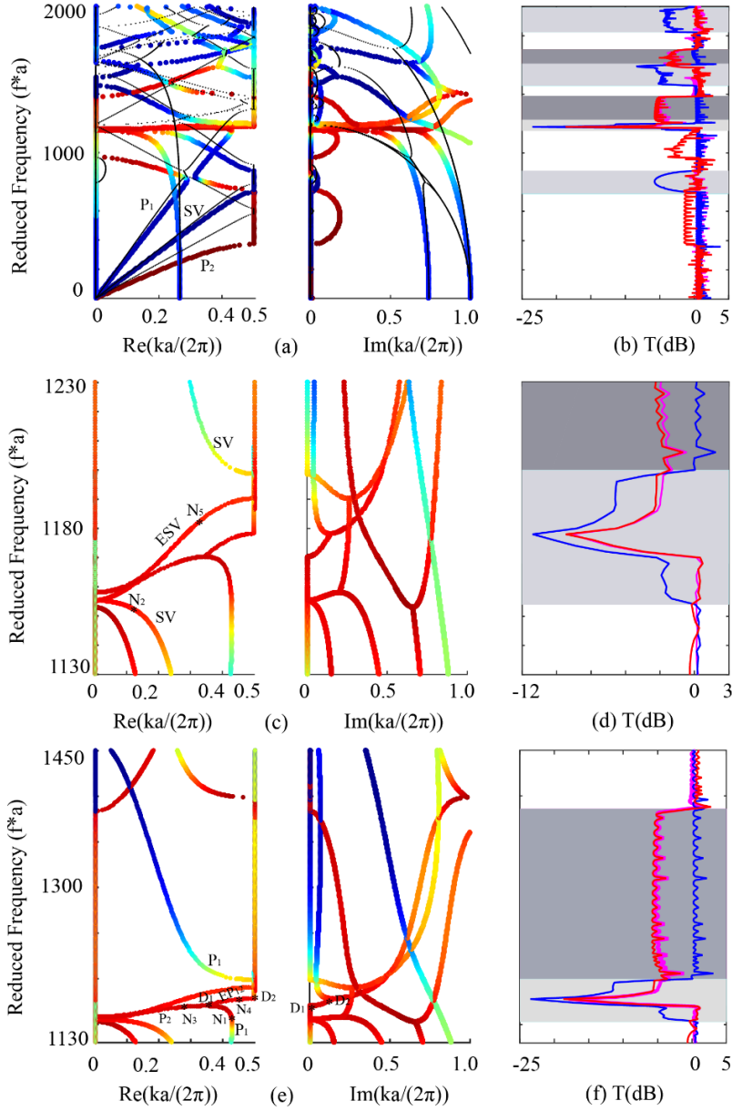
Figure 2: Complex band structures and transmission for the P/E system (elastic inclusion in a poroelastic matrix). Panel (a) consists of two parts: the left and right parts show the relation of the reduced frequency with the real and imaginary parts of the wave number, respectively. The color scale indicates wave polarization varying from blue (0) to red (1). Black dots are for the complex band structure of the P/P system with the open-pore interface. Panel (b) shows the transmission spectrum of a finite structure with 50 unit cells. The red, blue, and pink solid lines are for the responses to incident signals (1, 0, 0), (0, 1, 0), and (0, 0, 1), respectively. The light gray regions represent the band gaps for the SV wave in the complex band structure, whereas the gray regions show the band gaps for longitudinal waves. Panels (c-f) are the zoomed complex band structures and transmission in the reduced frequency regions 1130 m/s - 1230 m/s and 1130 m/s - 1450 m/s.
