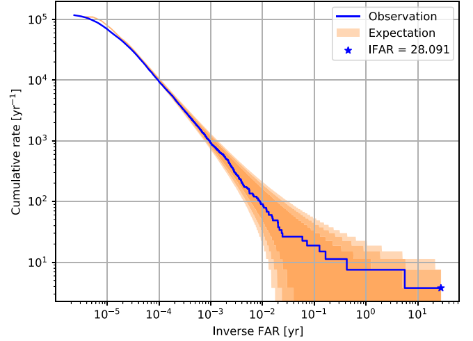
Figure 16. Modeling the turnover of the curve of the cumulative rate as a function of the IFAR in configuration n^{\circ}1 when we separate the associations by GBM spectral hardness and duration value.
