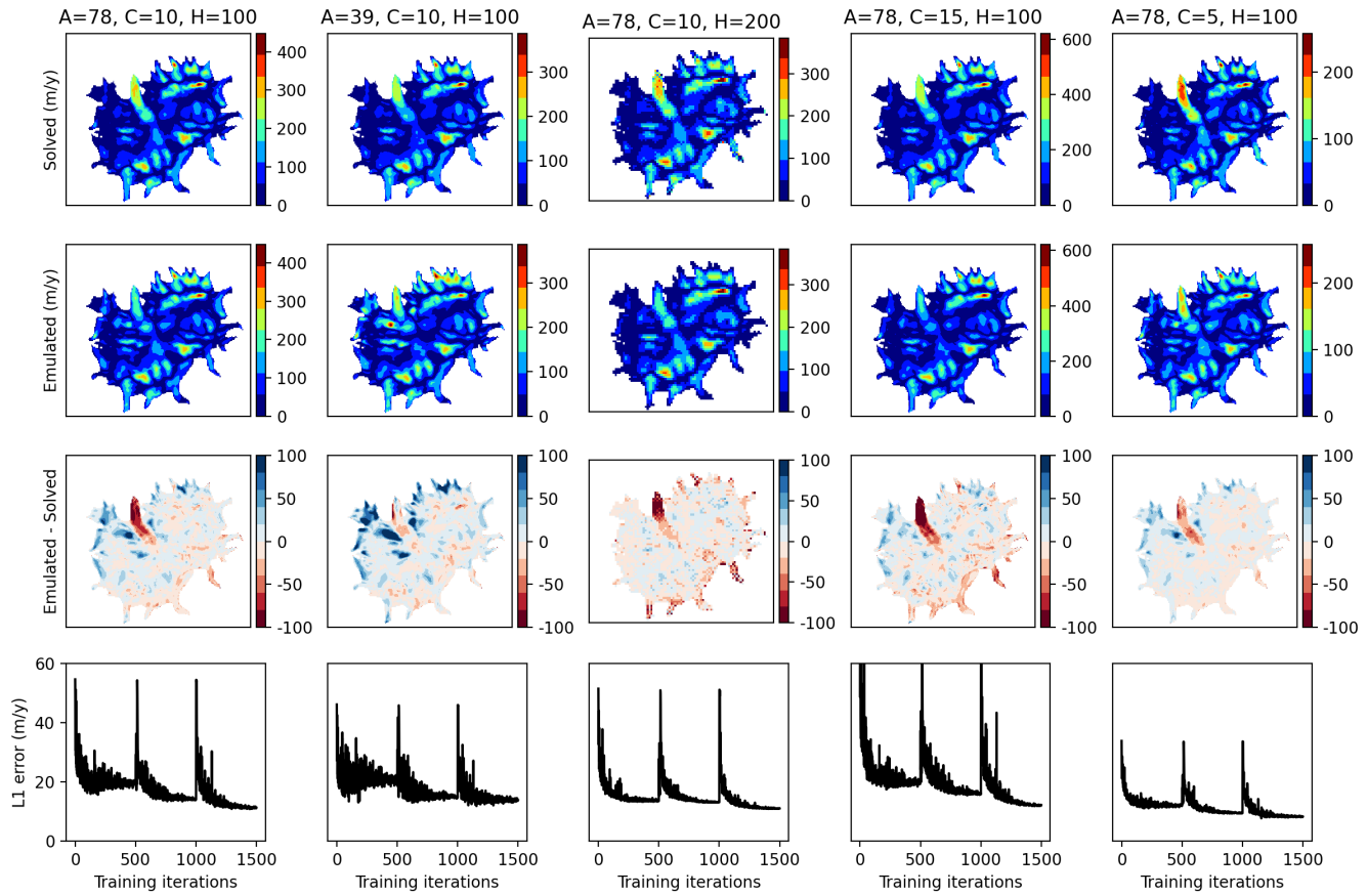
Fig. 15. Results of the emulator on the “test” glacier with varying values of A , c , and H . Each column corresponds to one parameter set ( A , c , H ) (the first column shows the default original parameters). The first row displays the “solved” surface ice flow solution. The second row displays the “emulated” solution after training over the glacier catalogue, while the third shows the difference between this solution and the “solved” one. The last row shows the L1 error through the training. The jumps each 5000 iterations are due to the re-initialization of the learning rate.
