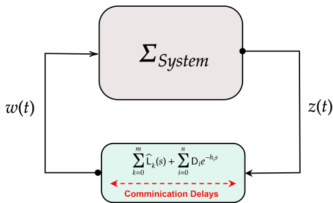
Fig. 1. Multi-agent nonlinear interconnected system with heterogeneous n constant and m distributed communication delays, where \hat{L}_k(s) and e^{-h_i s} are Laplace transform of L_k(t) the distributed density in [t - \tau_k, t] and the delta function \Delta_t(t - h_i) , respectively.
