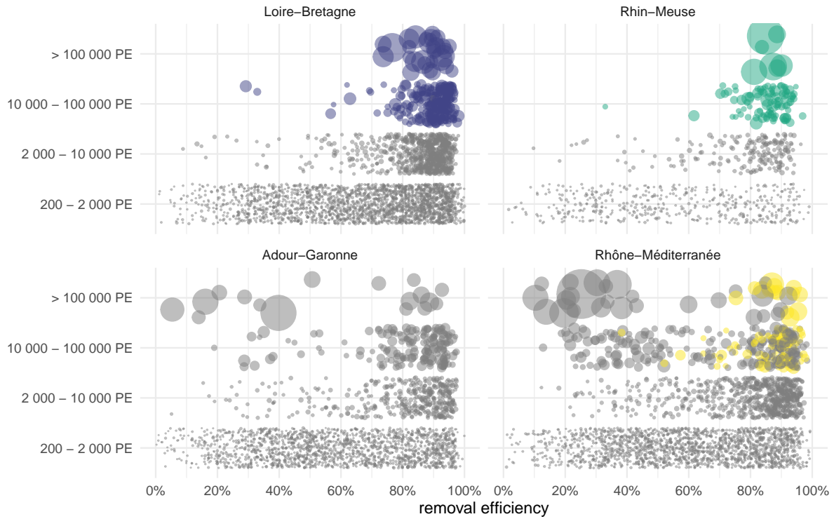
Figure 3: Individual WWTP N removal efficiencies, averaged over 2018-2020, in 4 of the French water agencies basins. Each dot is a WWTP, size is proportional to nominal capacity in population equivalent (PE). Dots are colored if the WWTP must reach minimal performances due to N sensitive area classification (see Figure 2a and text) or grey otherwise.
